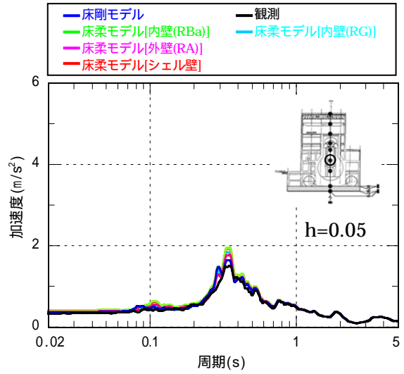
2階 (O.P. 18.7m)
