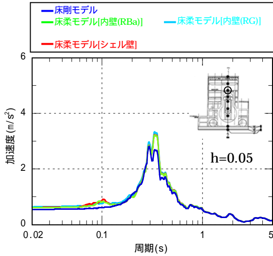
5階 (O.P. 39.92m)
