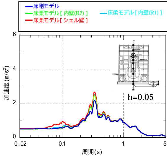
5階 (O.P. 39.92m)
