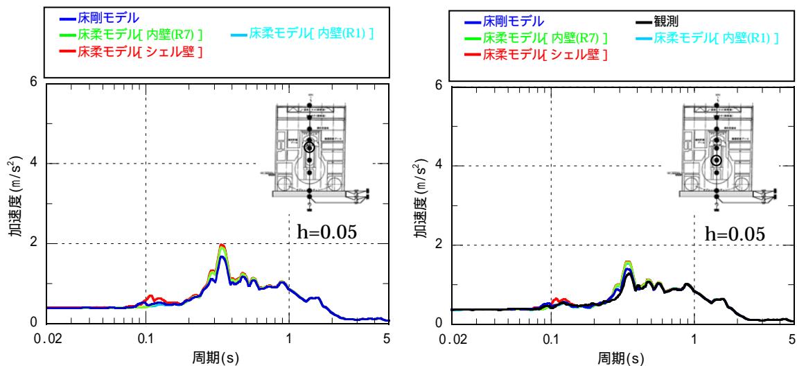
3階 (O.P. 26.9m)
