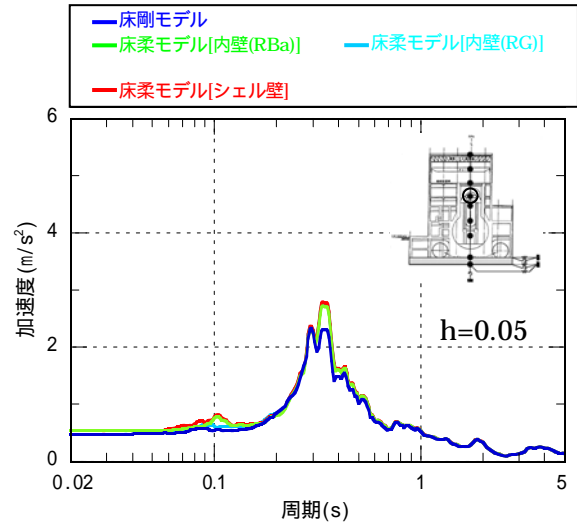
4階 (O.P. 32.3m)
