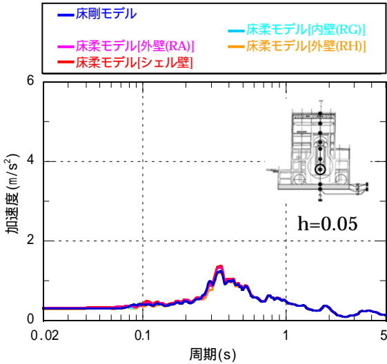
1階 (O.P. 10.2m)
