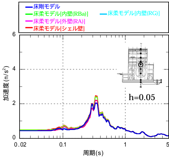
3階 (O.P. 26.9m)
