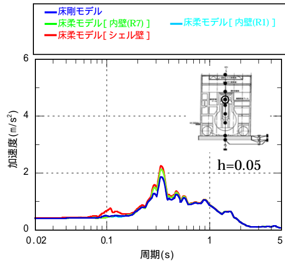
4階 (O.P. 32.3m)
