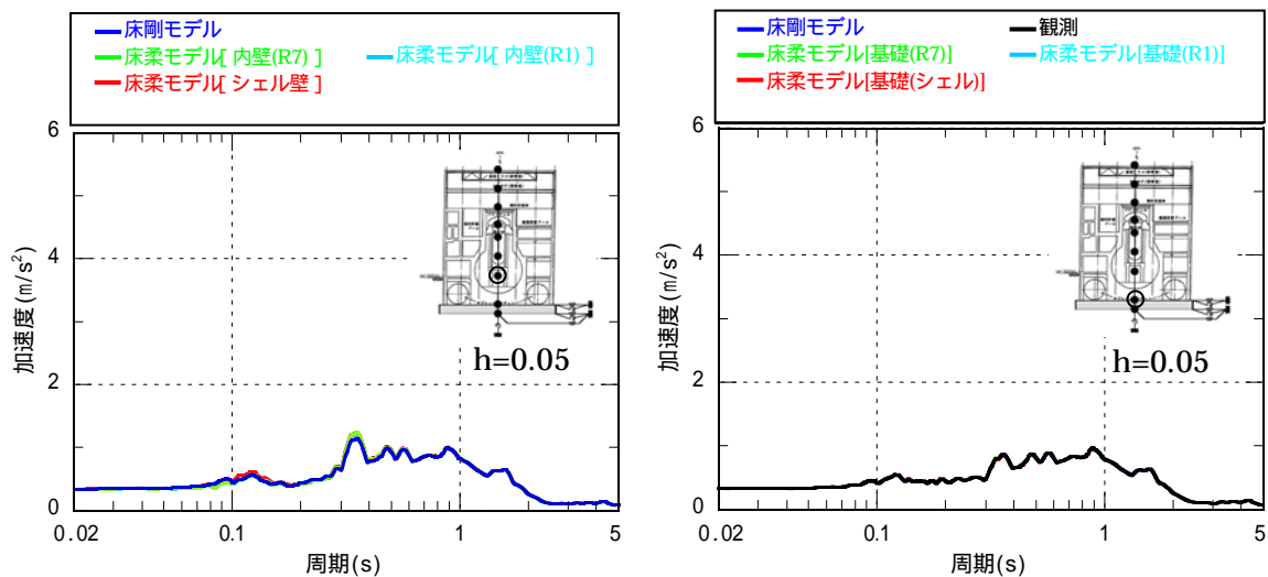
1階 (O.P. 10.2m)
