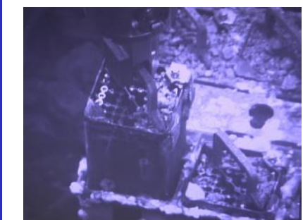
Fuel removal (April 15, 2019) (As of February 27, 2020)
