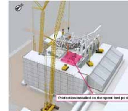
4. Simulated image of Unit 3 debris removal
