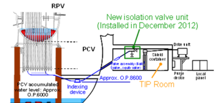
2. Overview of the TIP guide pipes
