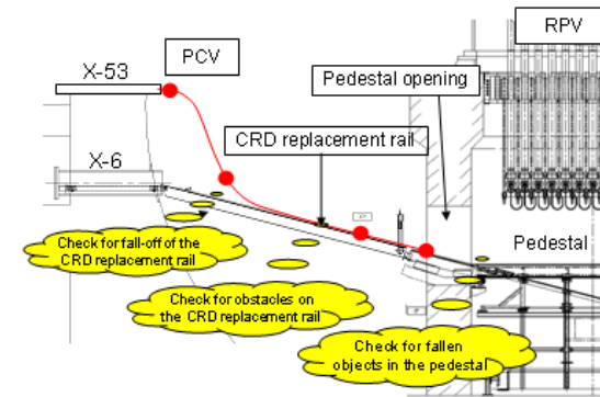
1. Overview of investigation of the inside of the PCV
