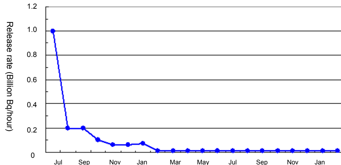
Release rate of radioactive material (cesium) per hour at Unit 1-3 Reactor Building
