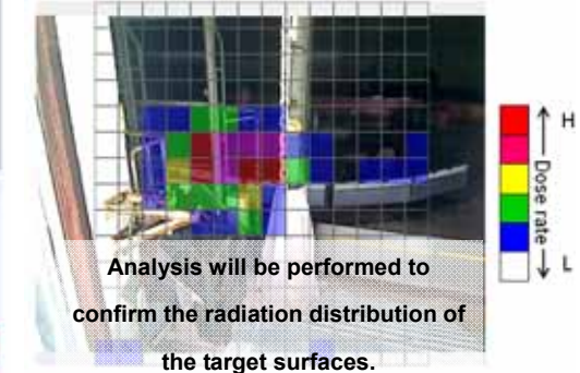
5. \gamma camera measurement results
