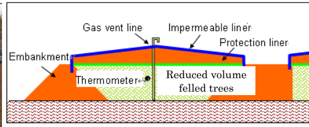
Overview of the temporary storage facility for felled trees (Embankment type)
