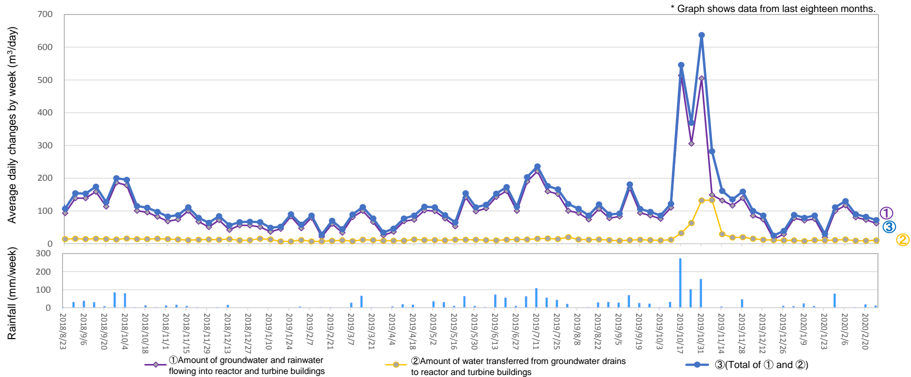
Amount of water transferred from groundwater drains to reactor and turbine buildings (From Feb 20, 2020 to Feb 26, 2020)
