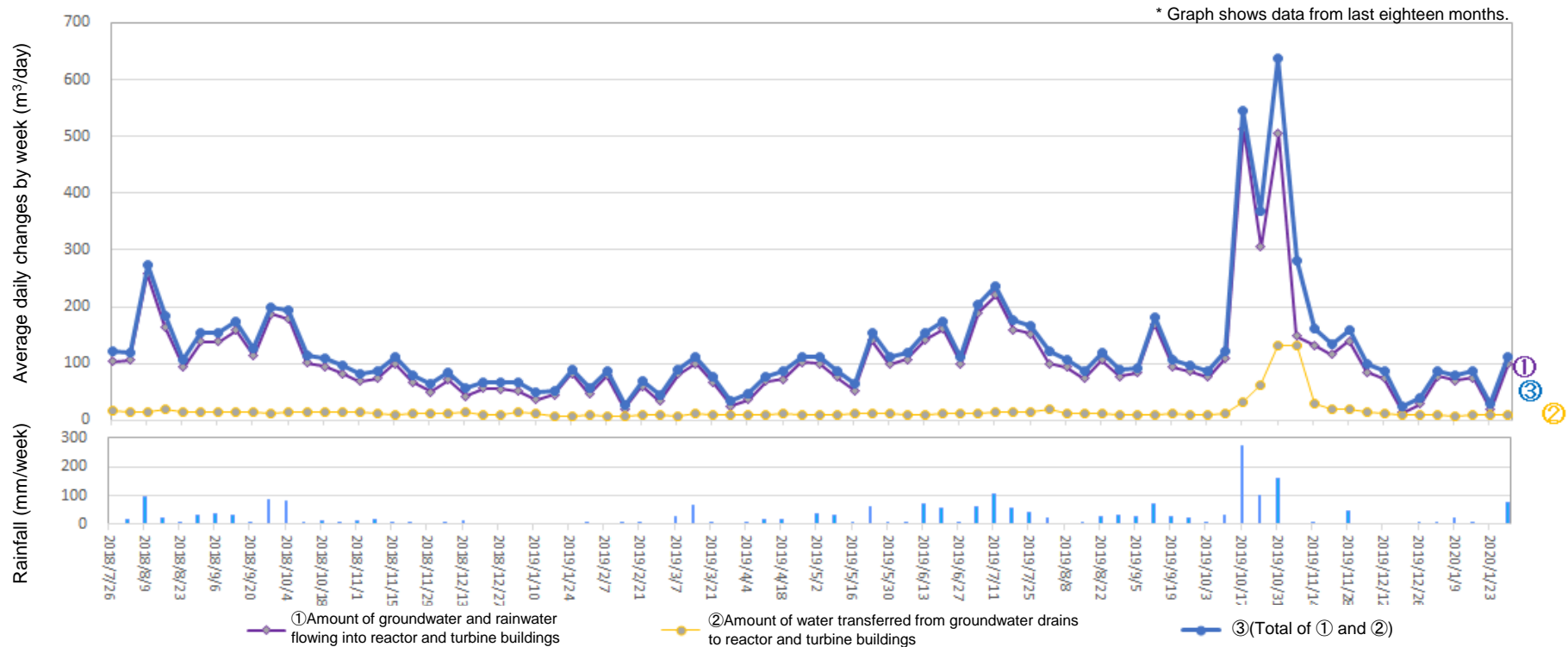
Amount of water transferred from groundwater drains to reactor and turbine buildings (From Jan 23, 2020 to Jan 29, 2020)
