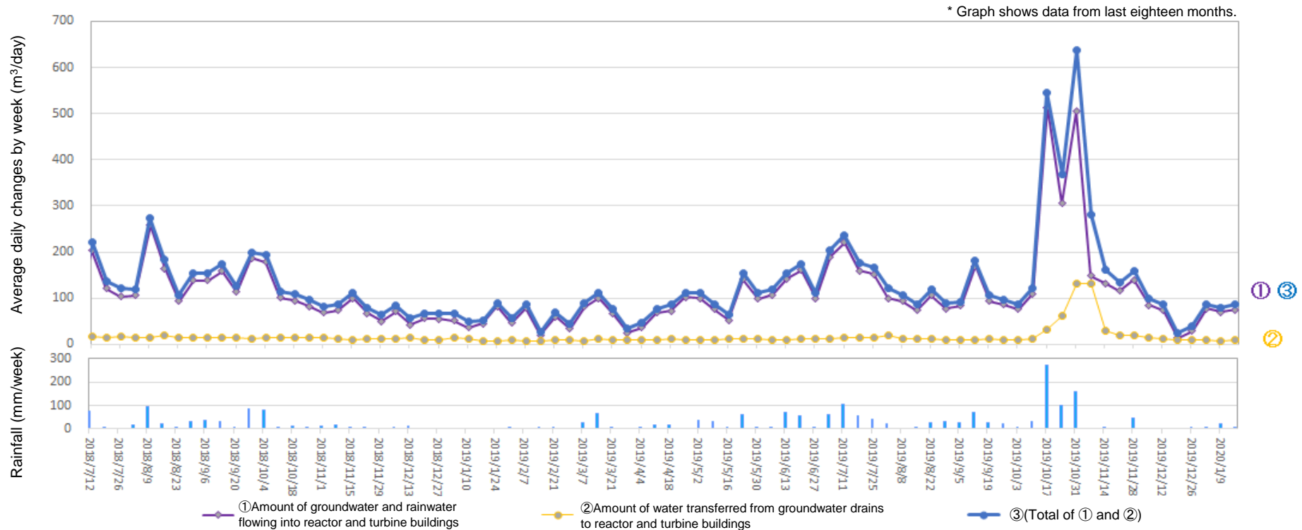
Amount of water transferred from groundwater drains to reactor and turbine buildings (From Jan 9, 2020 to Jan 15, 2020)
