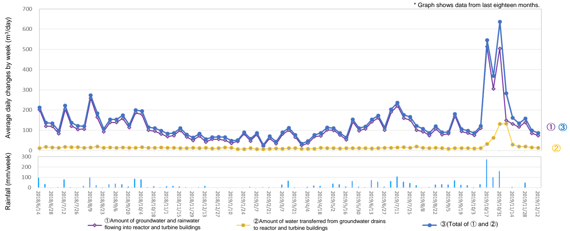
Amount of water transferred from groundwater drains to reactor and turbine buildings (From Dec 5, 2019 to Dec 11, 2019)
