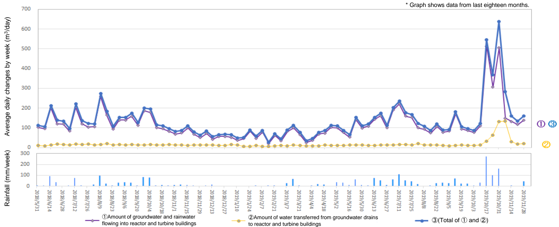
Amount of water transferred from groundwater drains to reactor and turbine buildings (From Nov 21, 2019 to Nov 27, 2019)
