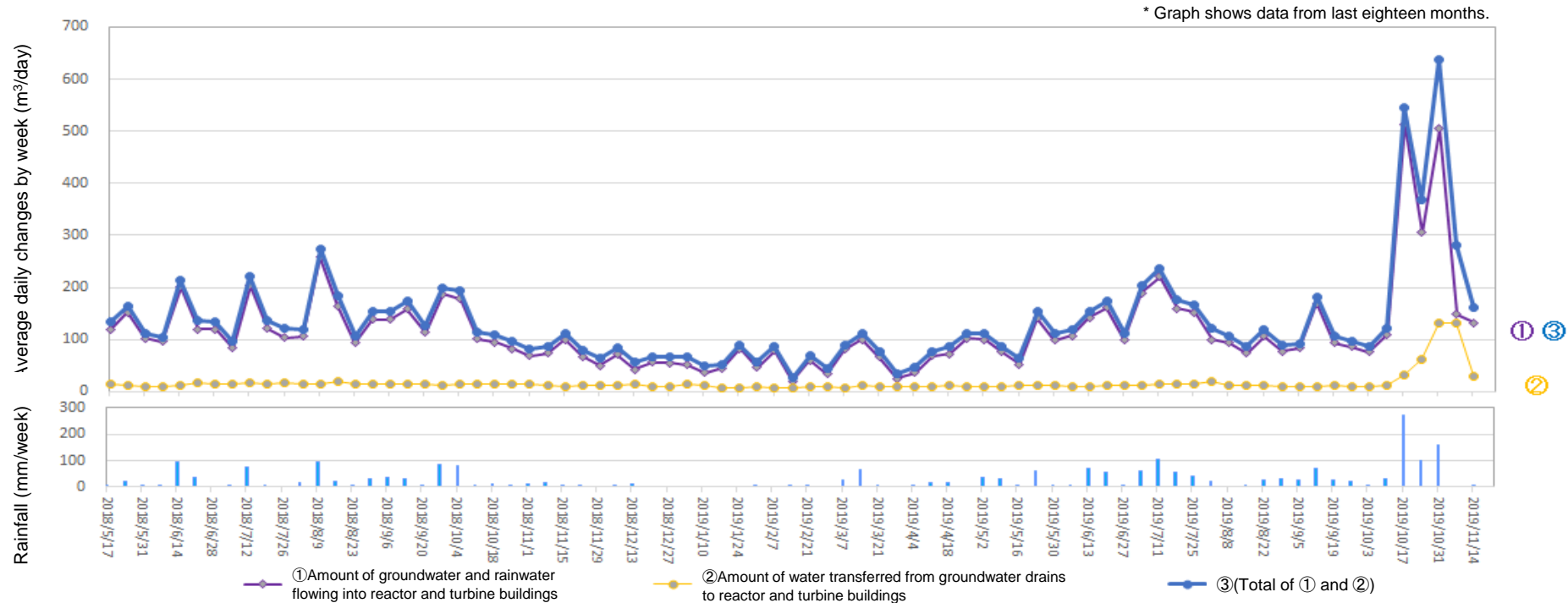
Amount of water transferred from groundwater drains to reactor and turbine buildings (From Nov 7, 2019 to Nov 13, 2019)
