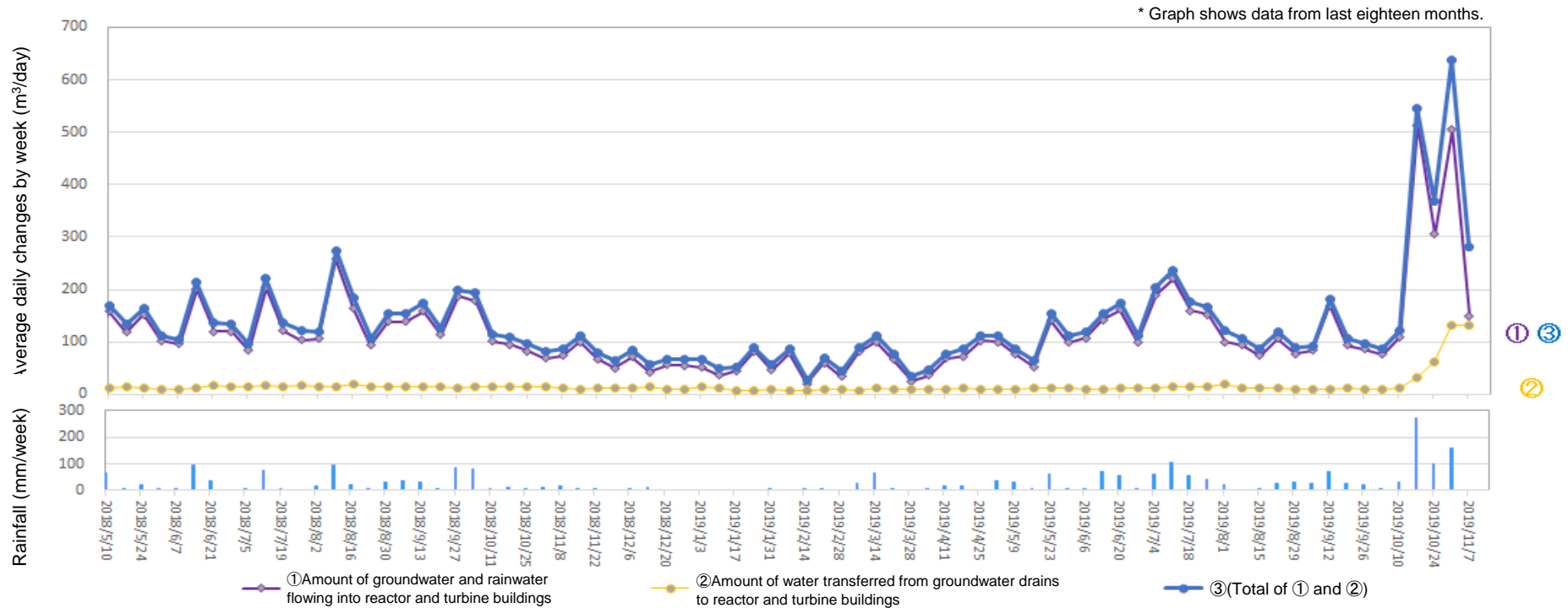
Amount of water transferred from groundwater drains to reactor and turbine buildings (From Oct 31, 2019 to Nov 6, 2019)
