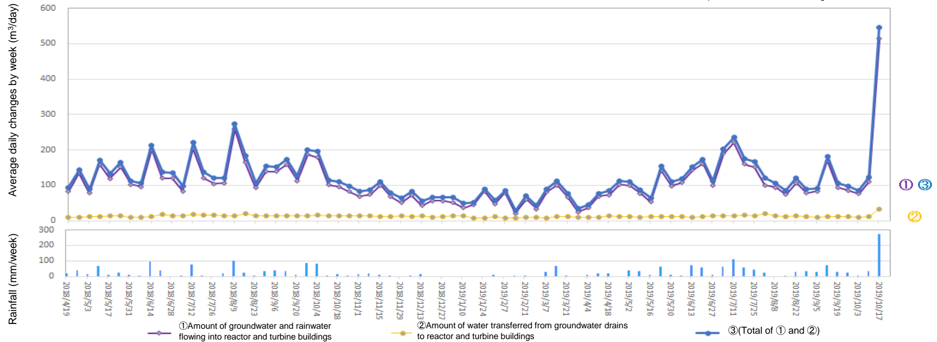
Amount of water transferred from groundwater drains to reactor and turbine buildings (From Oct 10, 2019 to Oct 16, 2019)
