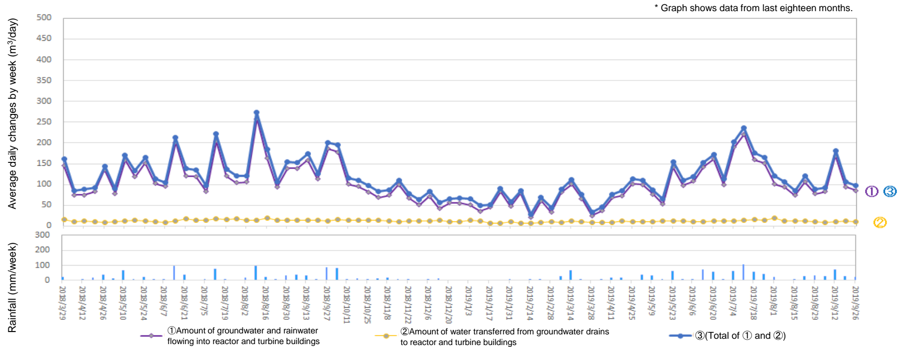
Amount of water transferred from groundwater drains to reactor and turbine buildings (From Sept 19, 2019 to Sept 25, 2019)
