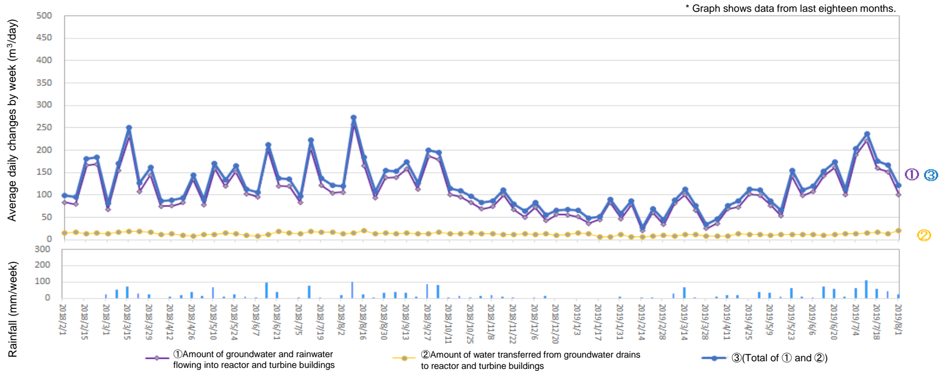
Amount of water transferred from groundwater drains to reactor and turbine buildings (From July 25, 2019 to July 31, 2019)
