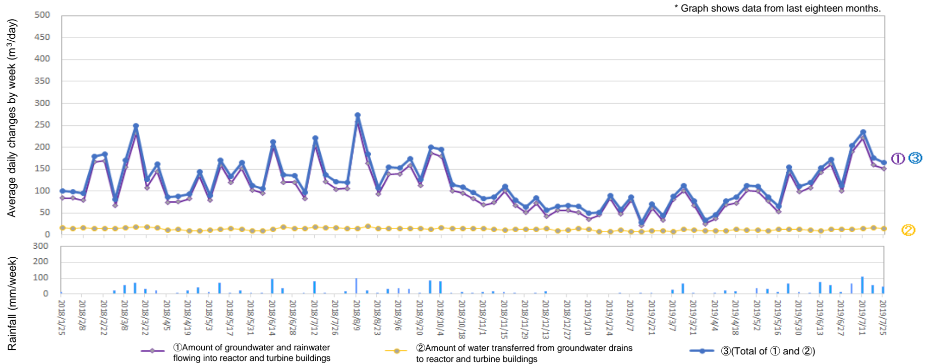
Amount of water transferred from groundwater drains to reactor and turbine buildings (From July 18, 2019 to July 24, 2019)
