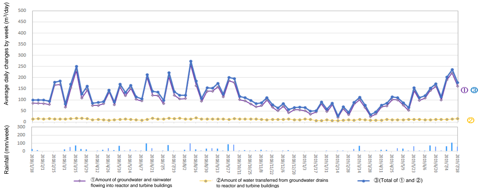
Amount of water transferred from groundwater drains to reactor and turbine buildings (From July 11, 2019 to July 17, 2019)
