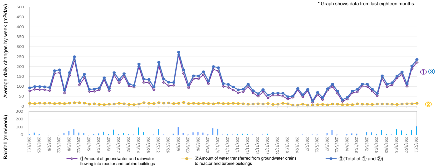
Amount of water transferred from groundwater drains to reactor and turbine buildings (From July 4, 2019 to July 10, 2019)
