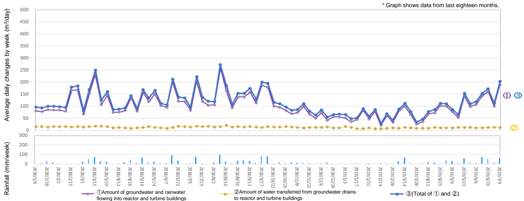
Amount of water transferred from groundwater drains to reactor and turbine buildings (From June 27, 2019 to July 3, 2019)
