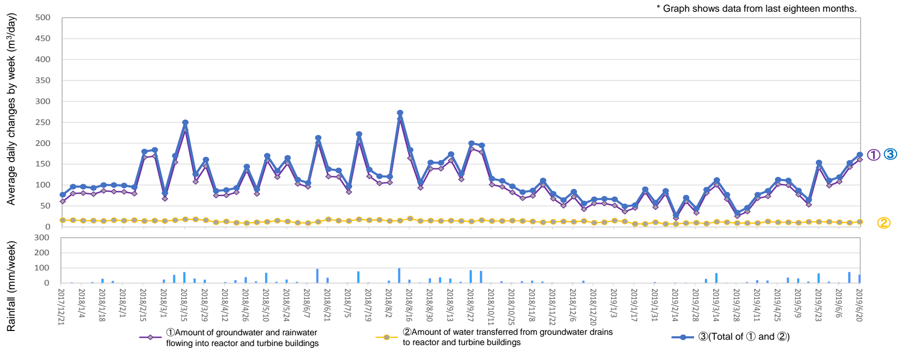
Amount of water transferred from groundwater drains to reactor and turbine buildings (From June 13, 2019 to June 19, 2019)
