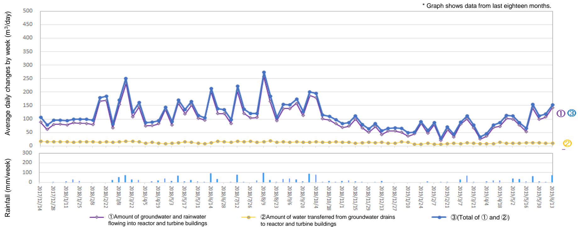
Amount of water transferred from groundwater drains to reactor and turbine buildings (From June 6, 2019 to June 12, 2019)
