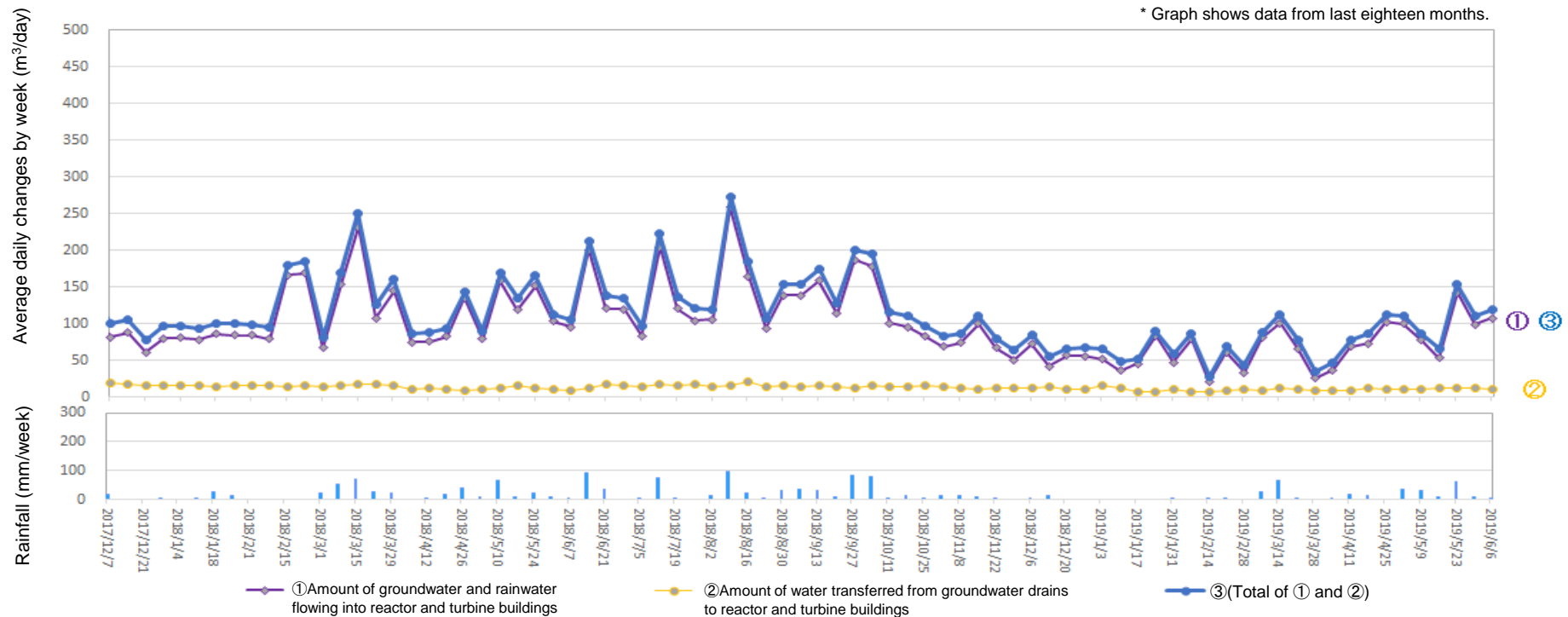
Amount of water transferred from groundwater drains to reactor and turbine buildings (From May 30, 2019 to June 5, 2019)
