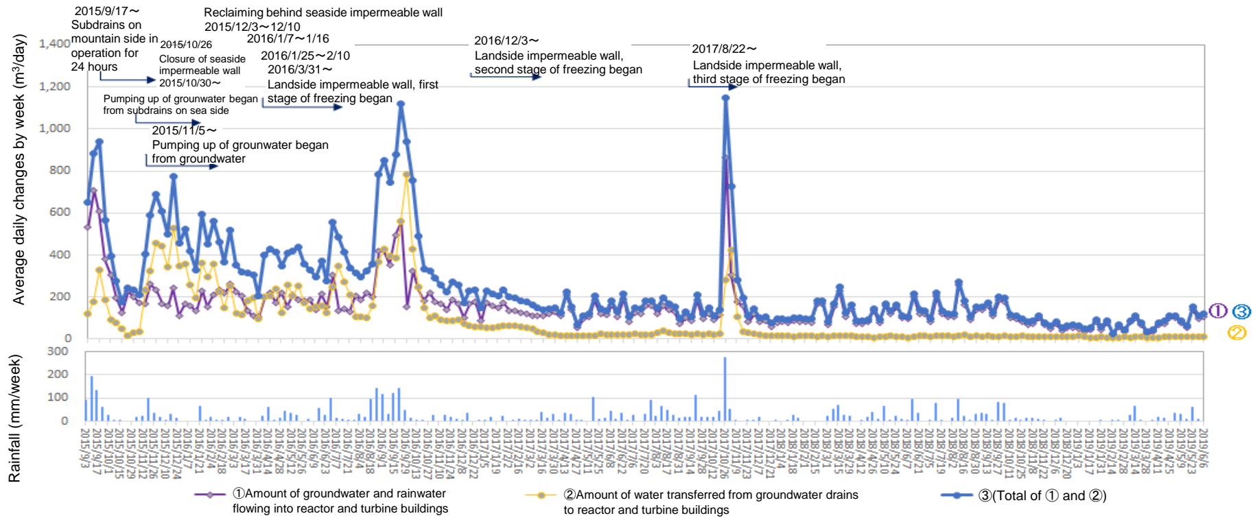
(Reference) Changes in the amount of water transferred from groundwater drains to reactor and turbine buildings and in the amount of groundwater and rainwater flowing into the buildings from the start of measurement
