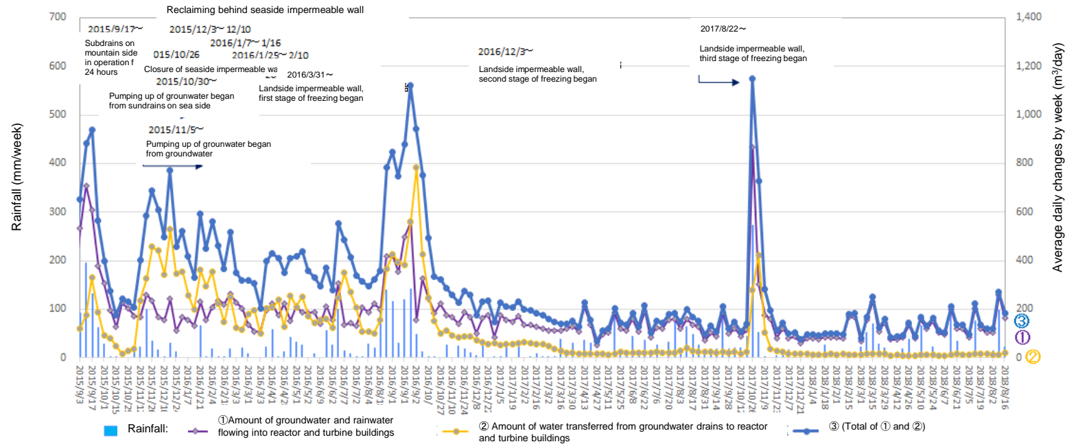
Amount of water transferred from groundwater drains to reactor and turbine buildings (From August 9, 2018 to August 15, 2018)
