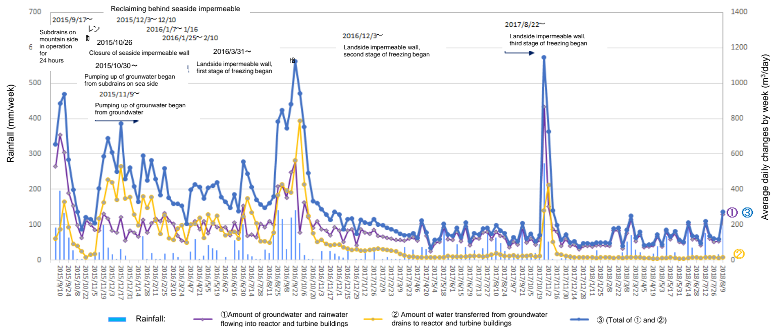
Amount of water transferred from groundwater drains to reactor and turbine buildings (From August 2, 2018 to August 8, 2018)
