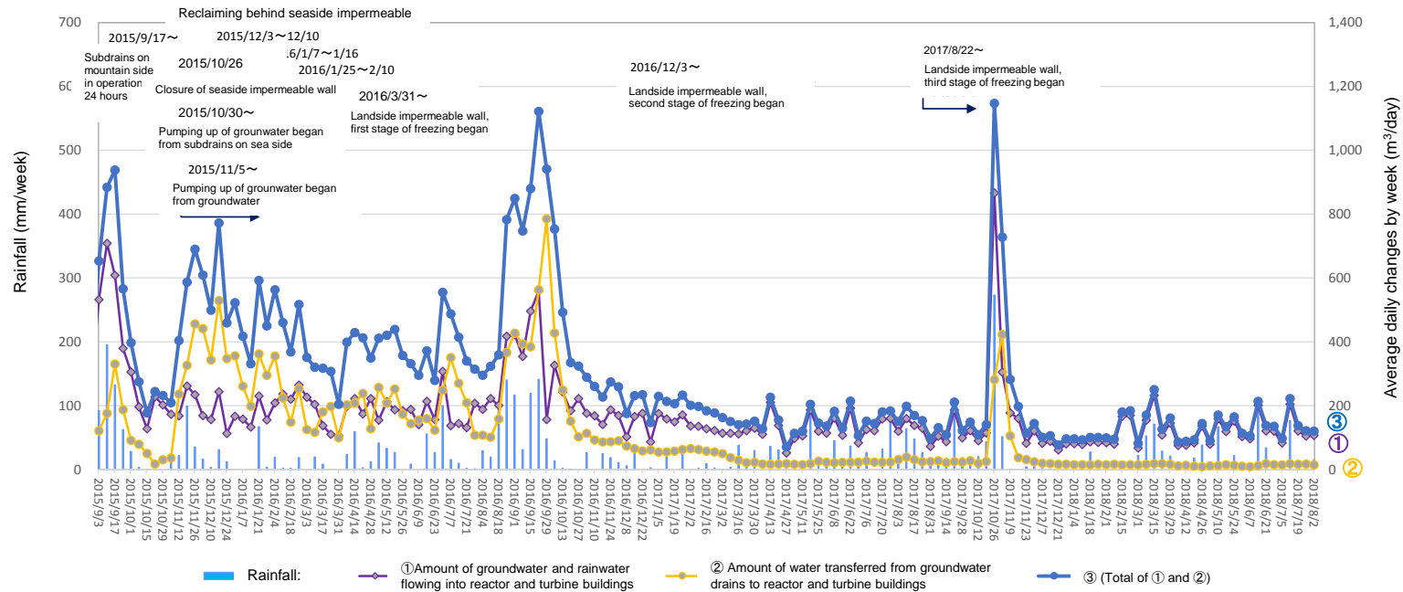
Amount of water transferred from groundwater drains to reactor and turbine buildings (From July 26, 2018 to August 1, 2018)
