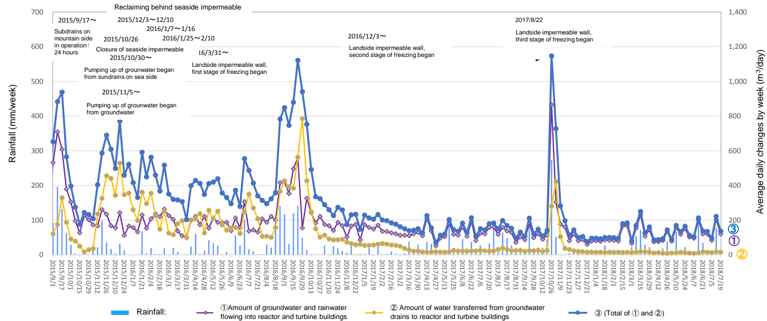
Amount of water transferred from groundwater drains to reactor and turbine buildings (From July 12, 2018 to July 18, 2018)
