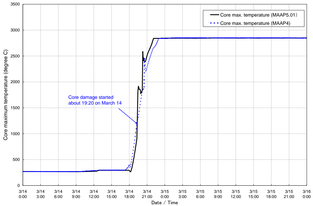
Figure 2-4 Core temperature changes of Unit-2
