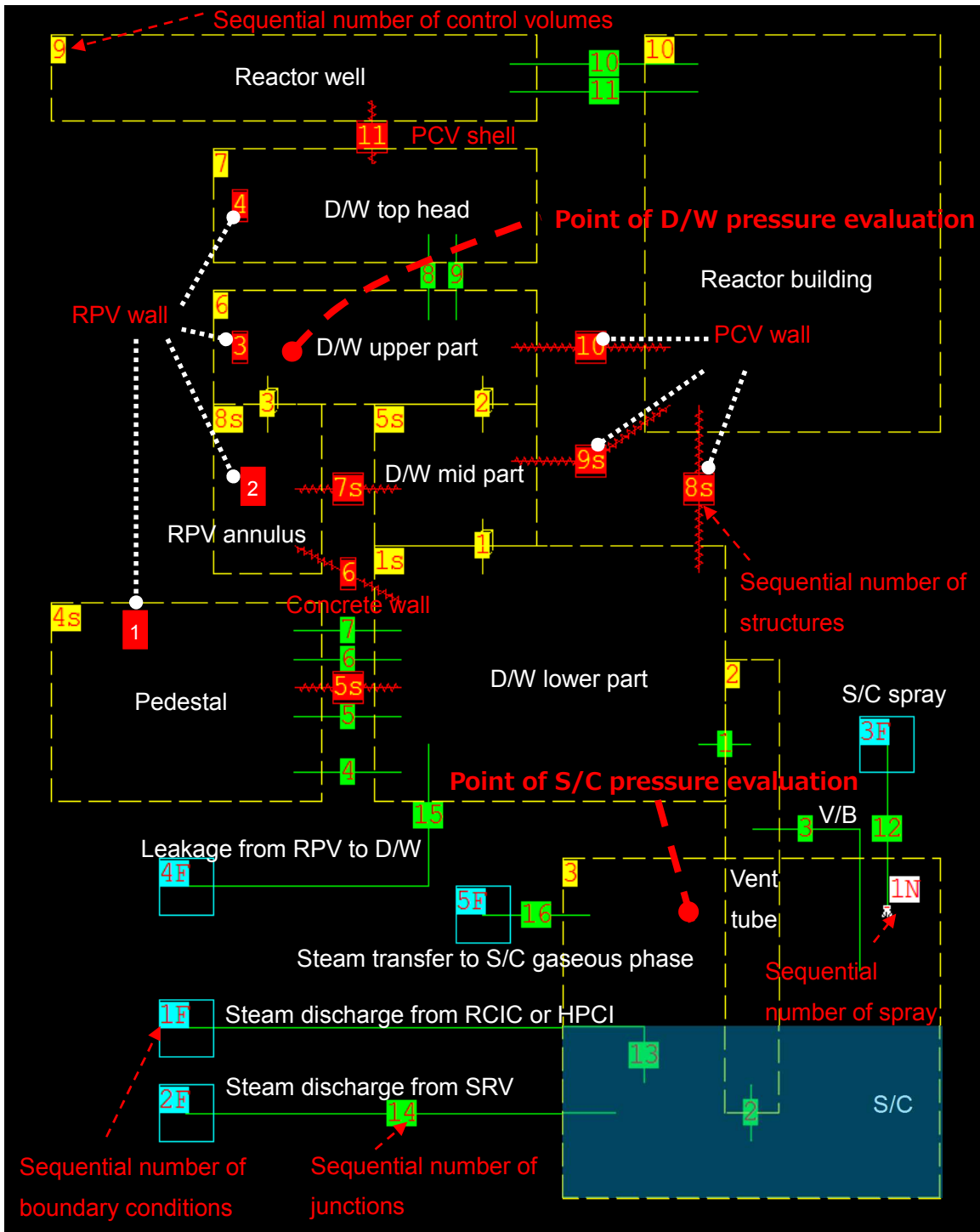
Figure 3-1 General geometry for GOTHIC analysis
