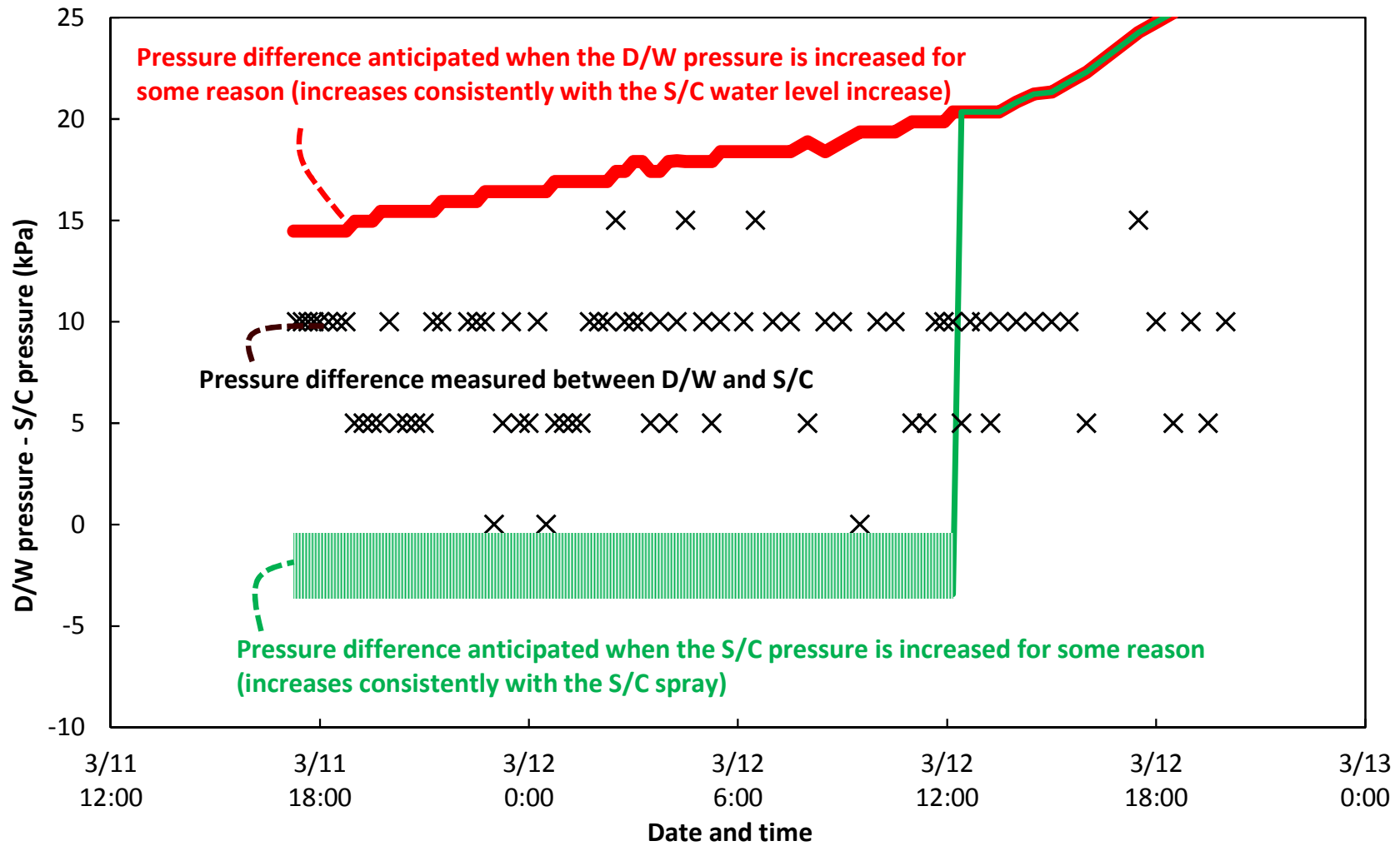
Figure 2-2 Difference between measured D/W and S/C pressures (D/W pressure – S/C pressure) on March 11 th to 12 th
