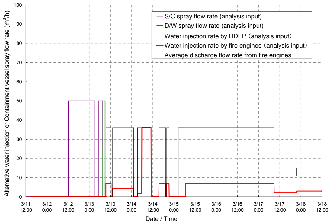
Figure 2 Water injection rates by fire engines and the containment vessel spray flow rate
