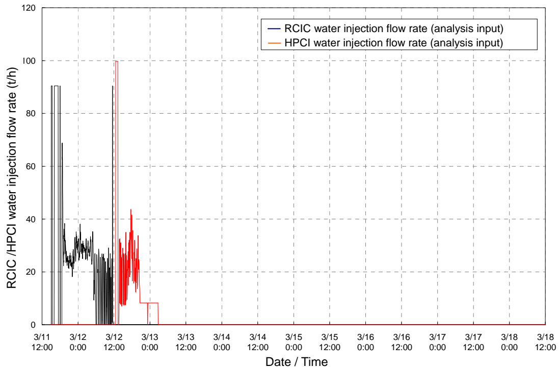
Figure 3 RCIC and HPCI water injection flow rates
