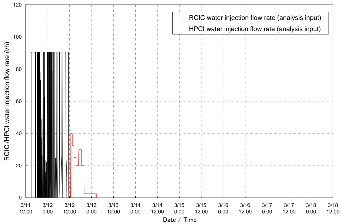
Figure 1 RCIC and HPCI water injection flow rates
