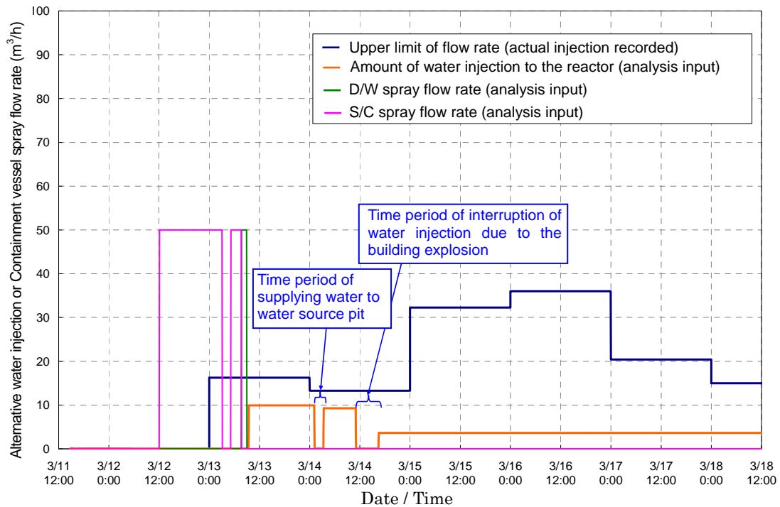
Figure 4 Water injection rates by fire engines and the containment vessel spray flow rate
