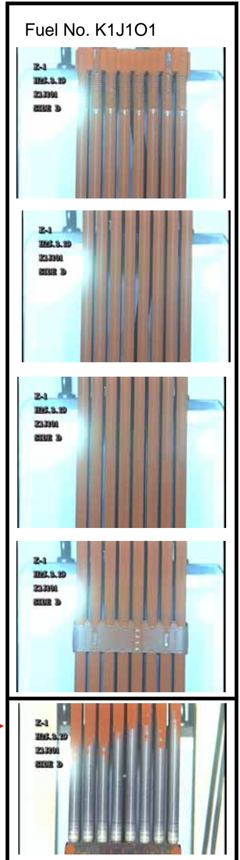
Overview of the bent fuel assembly water rods found at Unit 1 at Kashiwazaki-Kariwa Nuclear Power Station
