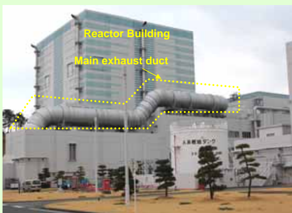
1. Outer appearance of Unit 4 main exhaust duct (Photo taken on April 5, 2012)
