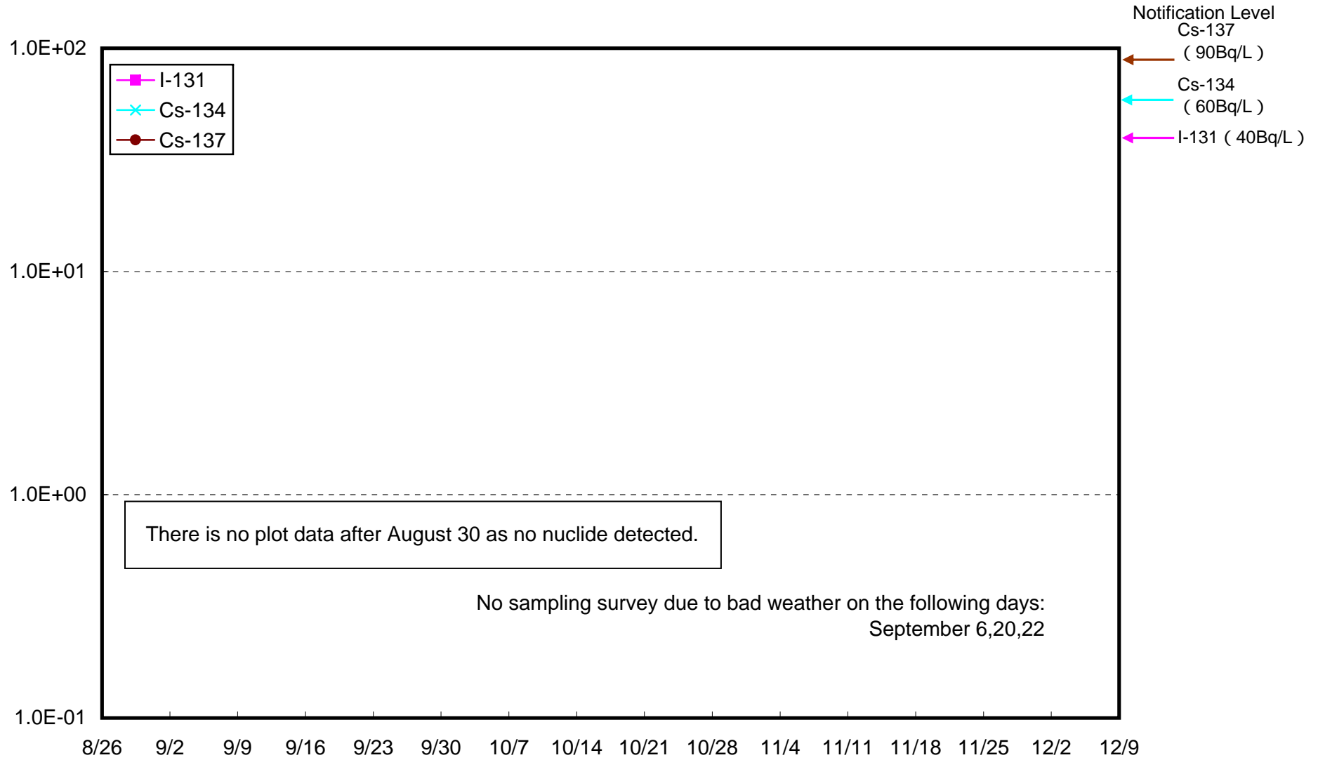
Radioactivity Density of Seawater around approx. 5 km offshore of Kashima City Upper Layer (Bq/L)
