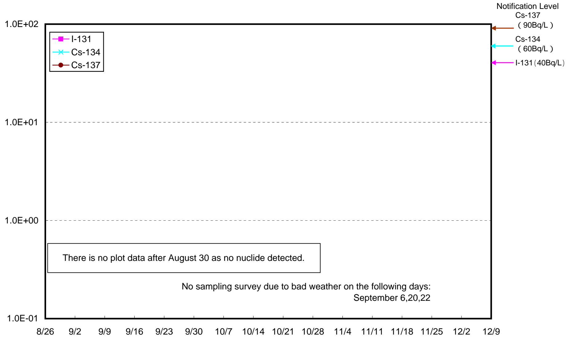
Radioactivity Density of Seawater around approx. 5 km offshore of Kashima City Lower Layer (Bq/L)
