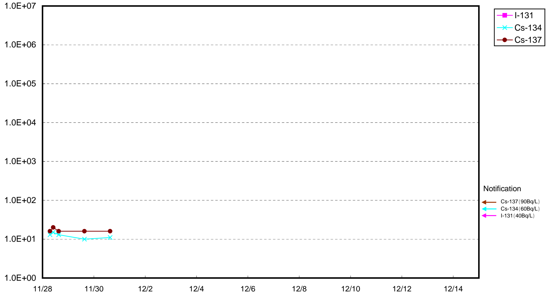
Radioactivity Density of Seawater at Units 5 Water Intake of Fukushima Daiichi NPS (Bq/ L)
