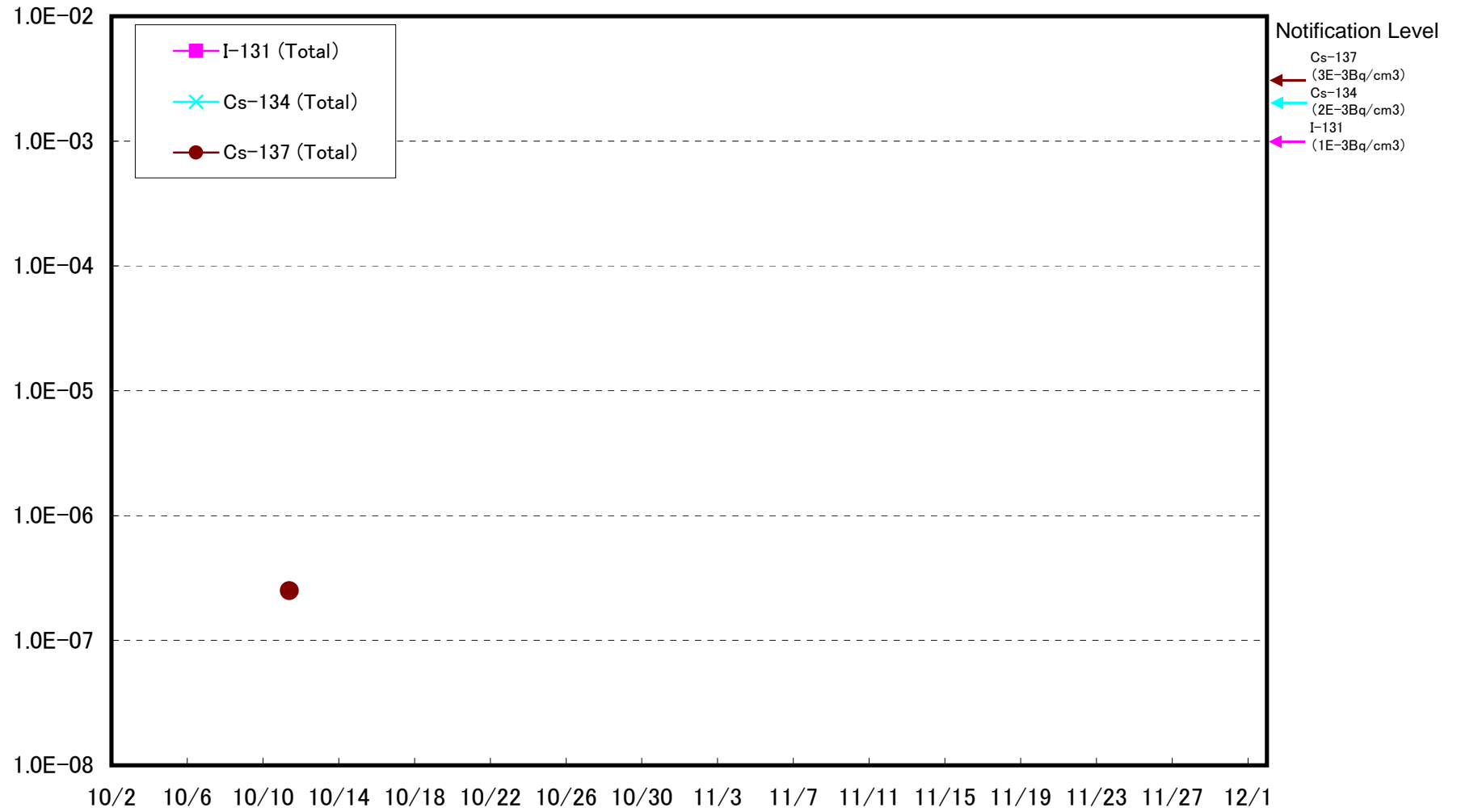
MP-8 of Fukushima Daiichi Results of Dust Nuclide Analysis (Bq/cm 3 )
