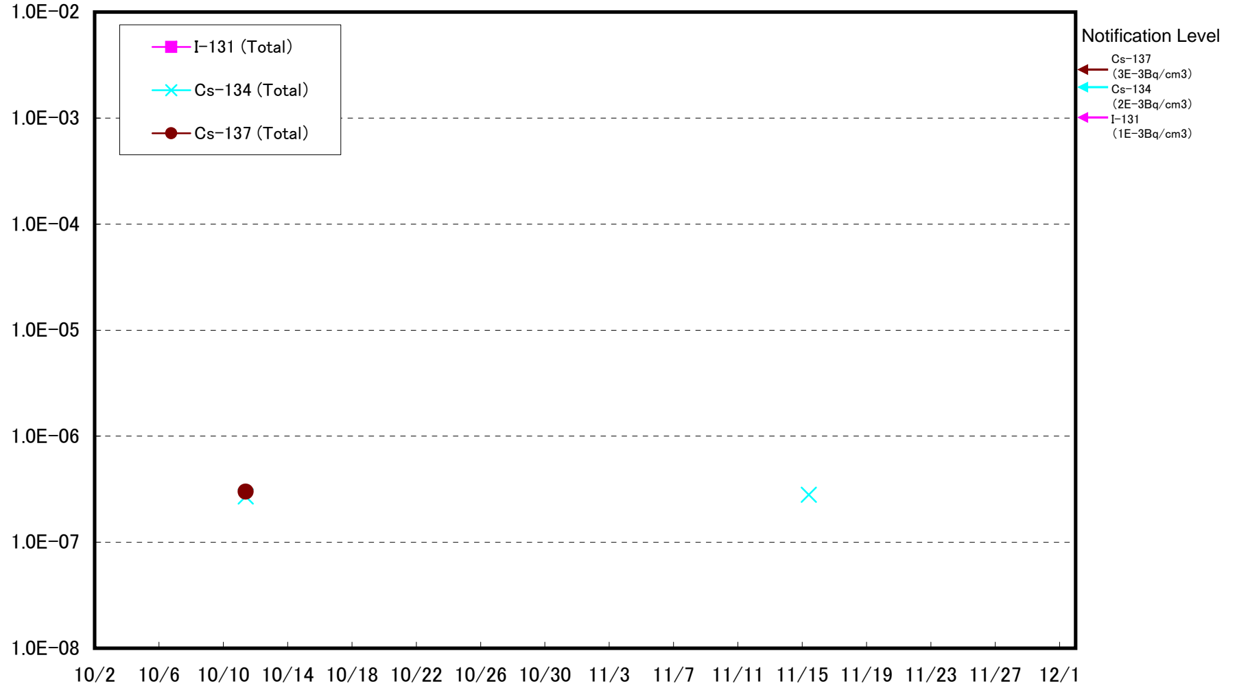
MP-3 of Fukushima Daiichi Results of Dust Nuclide Analysis (Bq/cm 3 )
