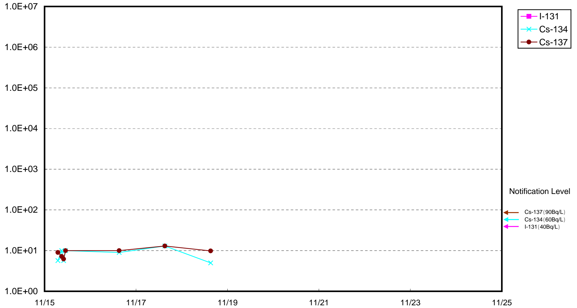
Radioactivity Density of Seawater at Fukushima Daiichi Power Plant unit 6 intake (Bq/L)
