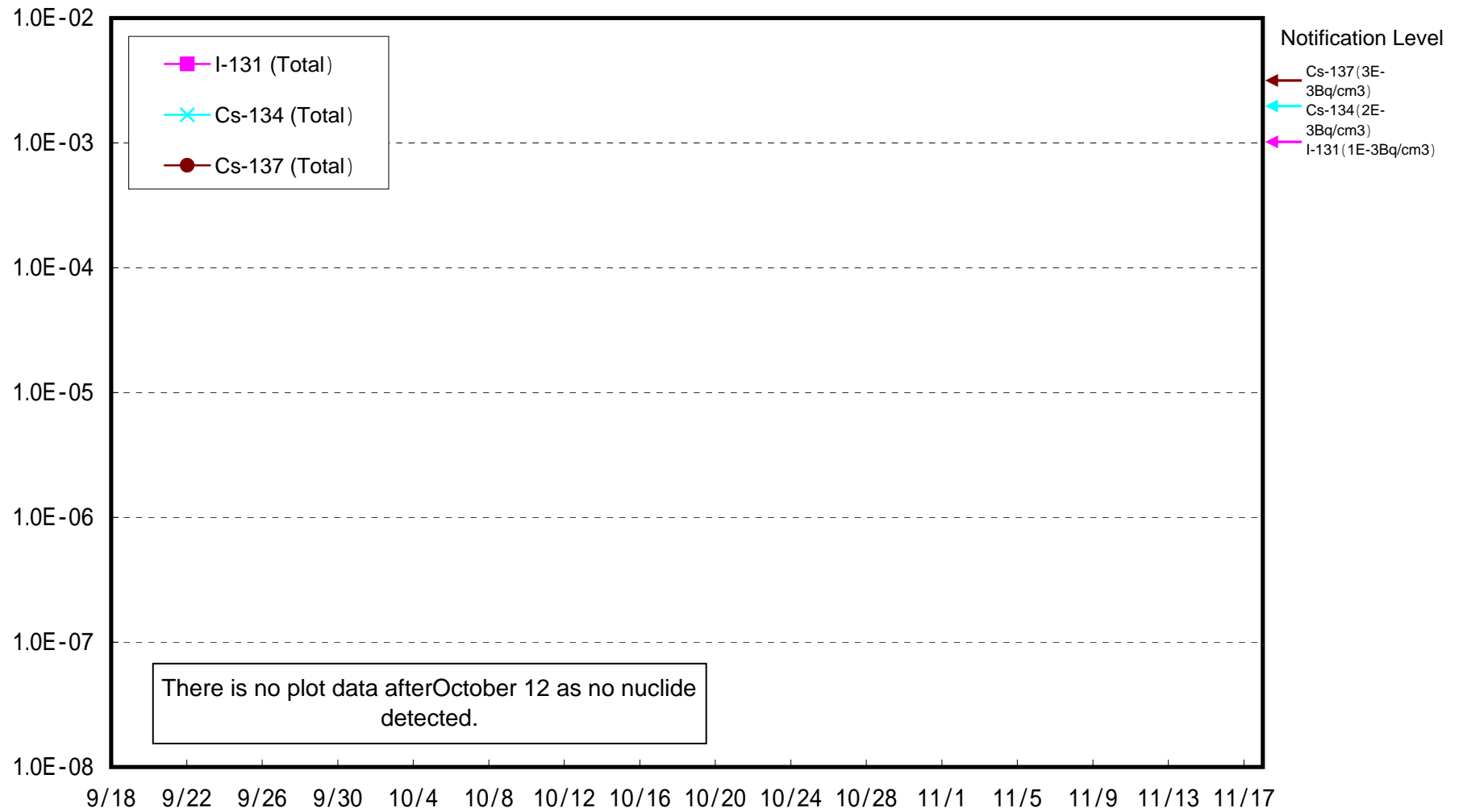
Water Treatment Building of Fukushima Daiichi Results of Dust Nuclide Analysis (Bq/cm 3 )
