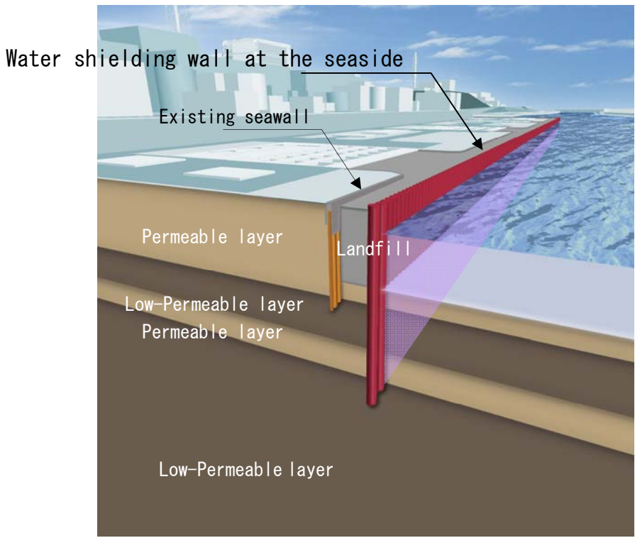
Cross-section view
