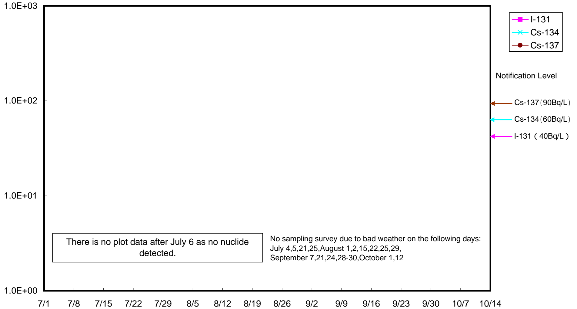
Radioactivity Density of Seawater approx. 15 km offshore of Hirono Town Upper Layer(Bq/L)
