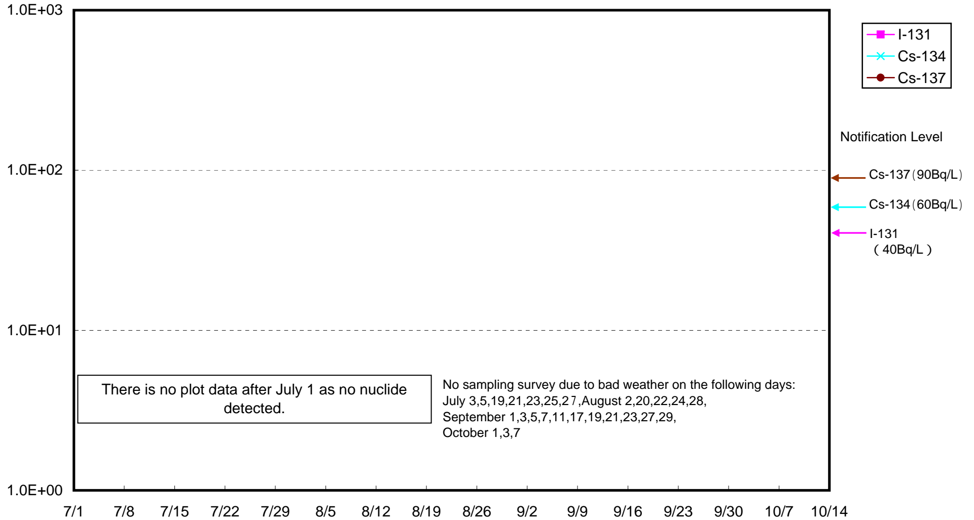
Radioactivity Density of Seawater 3km Offshore of Odaka Ward Lower Layer (Bq/L)
