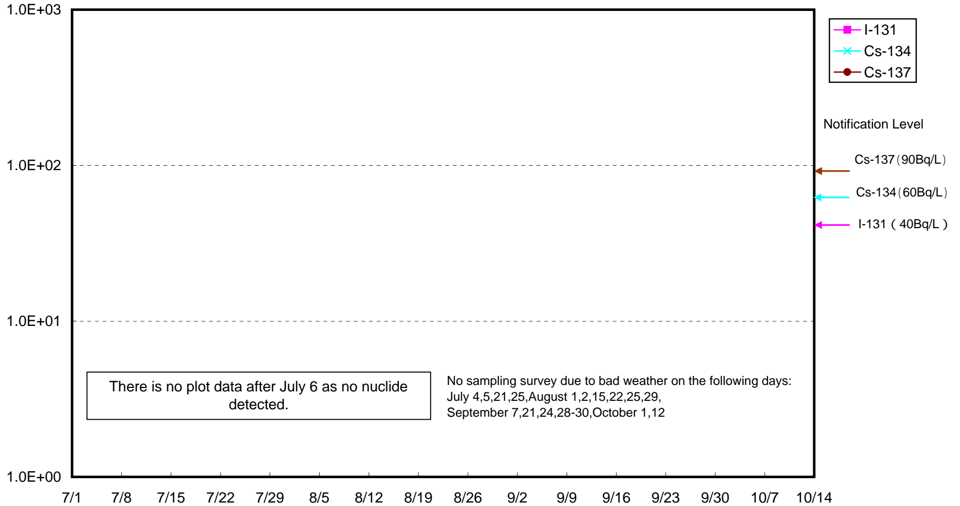
Radioactivity Density of Seawater approx. 15 km offshore of Iwasawa Shore Lower Layer (Bq/L)
