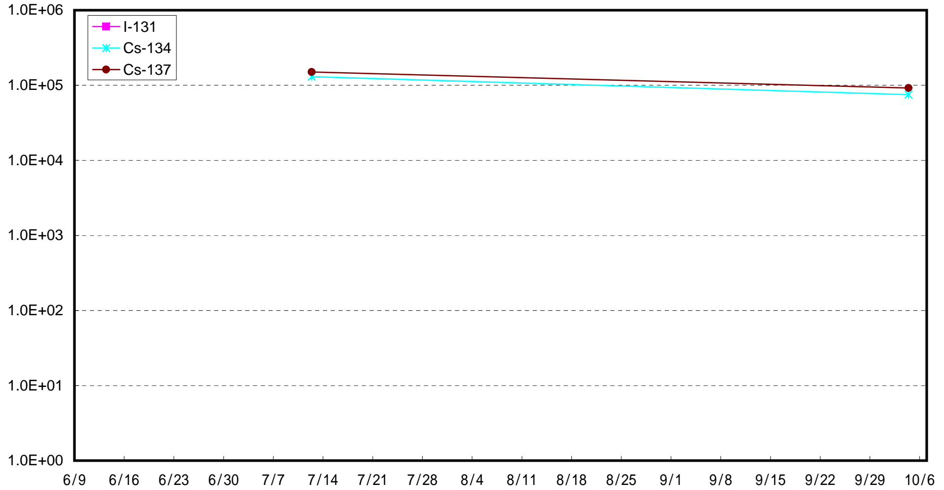
Radioactivity Density of the Ocean Soil at Shallow Draft Quay ( B q / k g )
