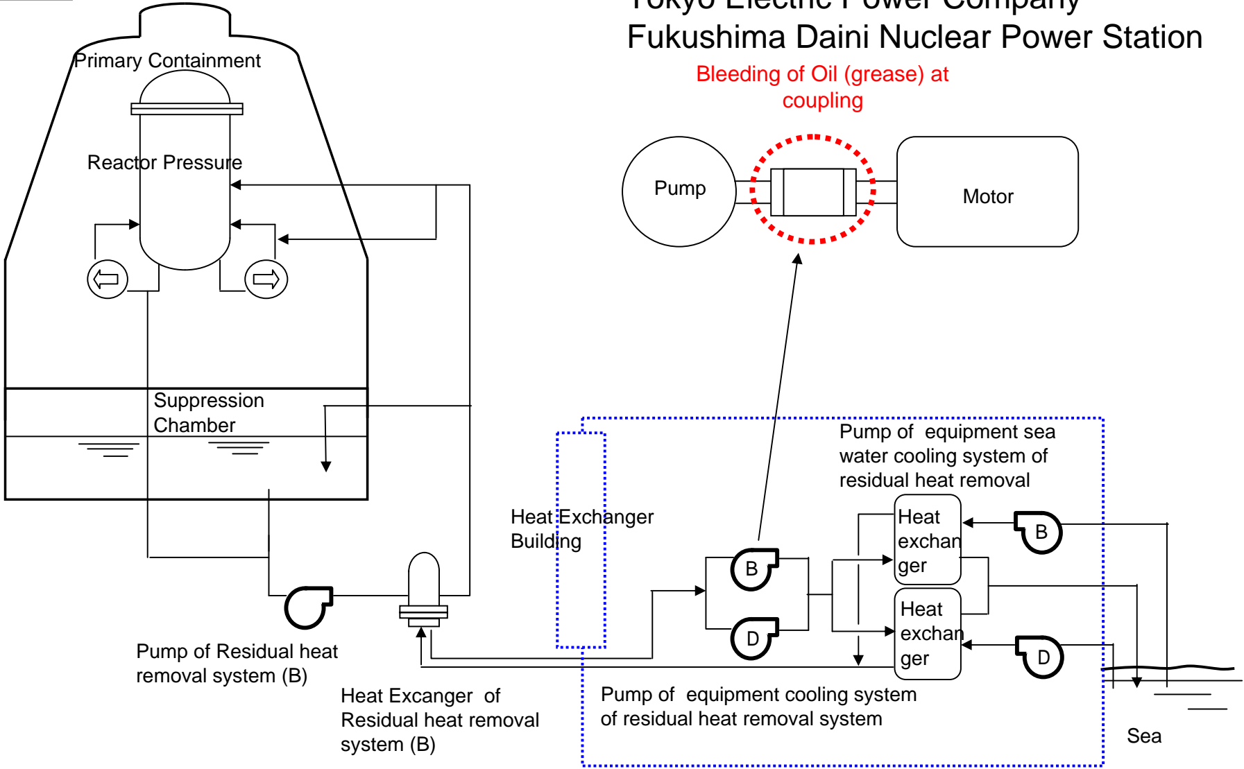
Layout of Residual heat removal system (B) of Unit 1 at Fukushima Daini Nuclear Power Station
