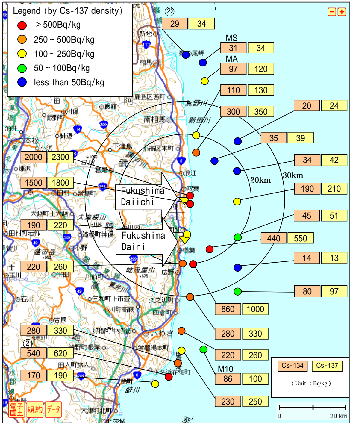
Readings of Additional Sea Area Monitoring at offshore of Fukushima Prefecture -marine soil- (September 8– 25,2011)
