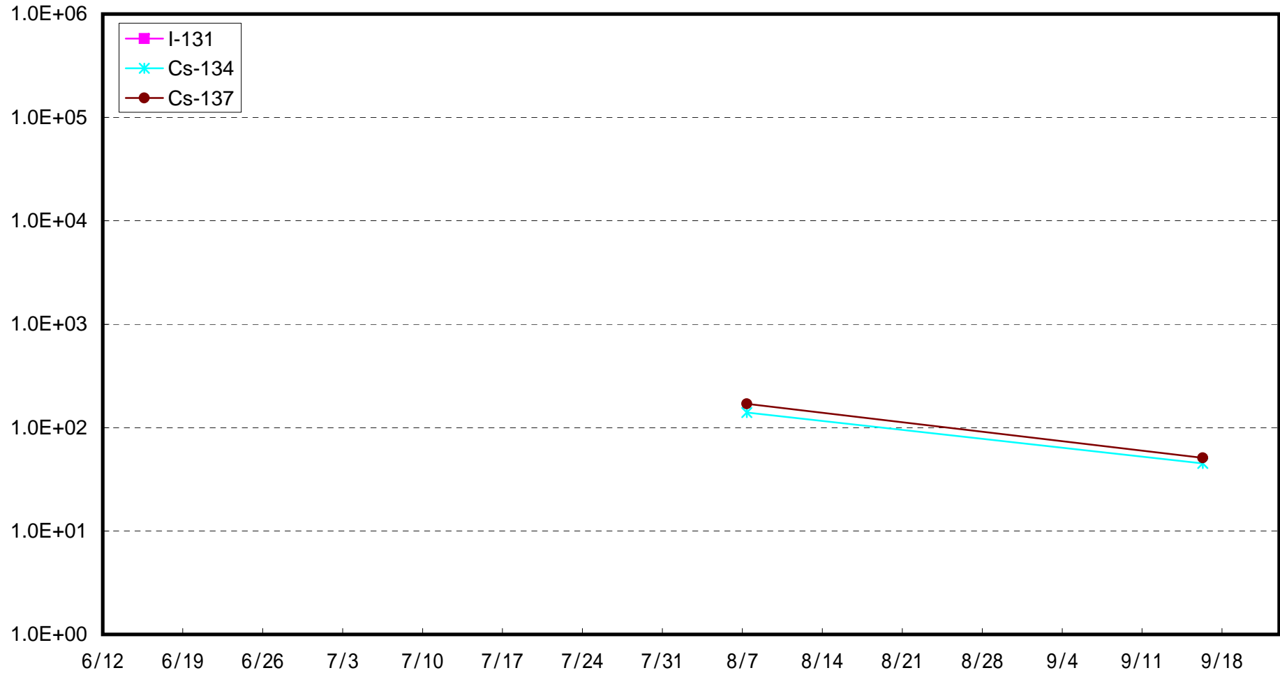
Radioactivity Density of Ocean Soil at 15 km Offshore of Fukushima Daini (Bq/kg)
