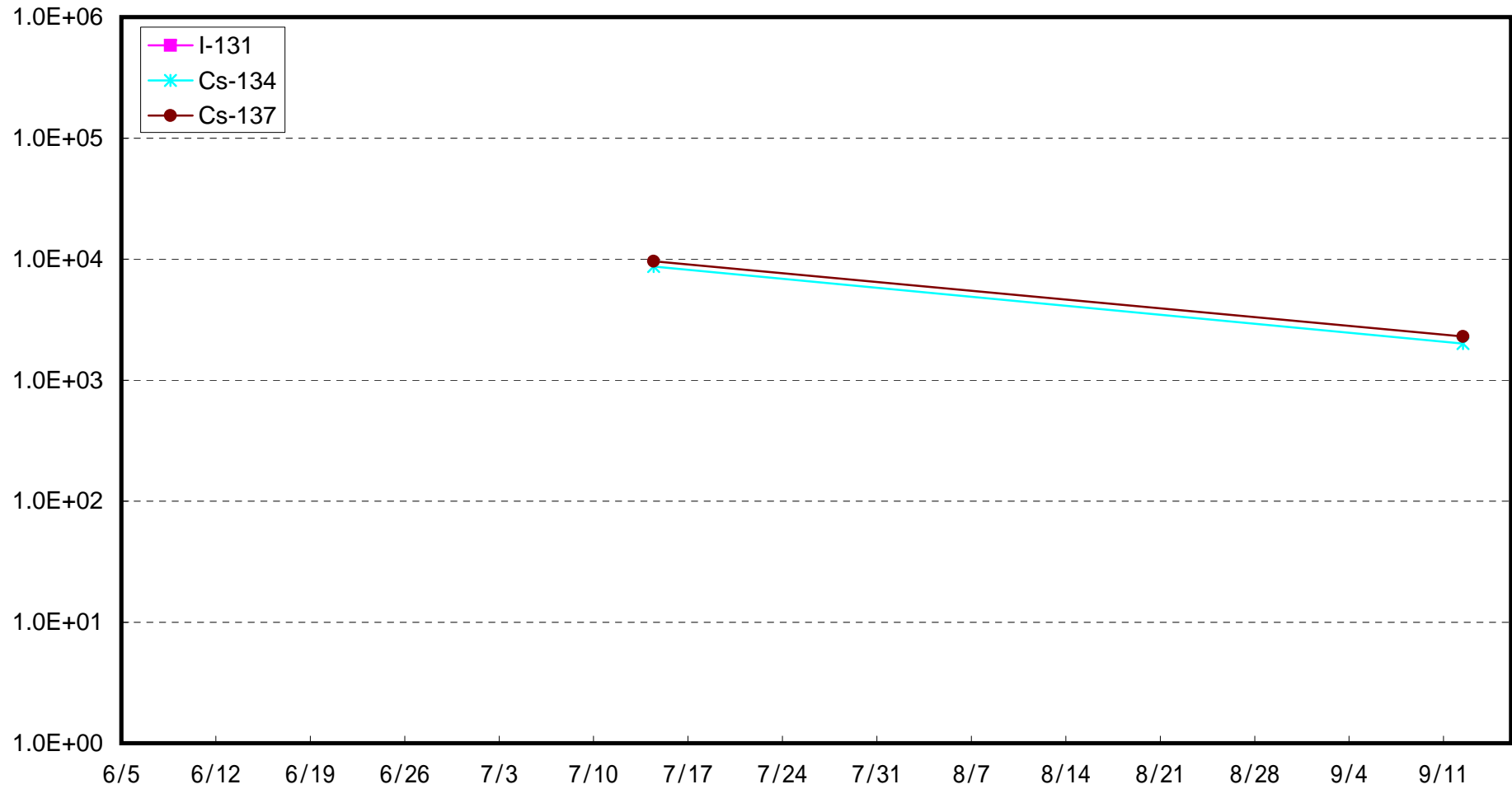
Radioactivity Density of Ocean Soil at North Discharge Channel of 1F (Around 5,6u Discharge Channel) (Bq/kg)
