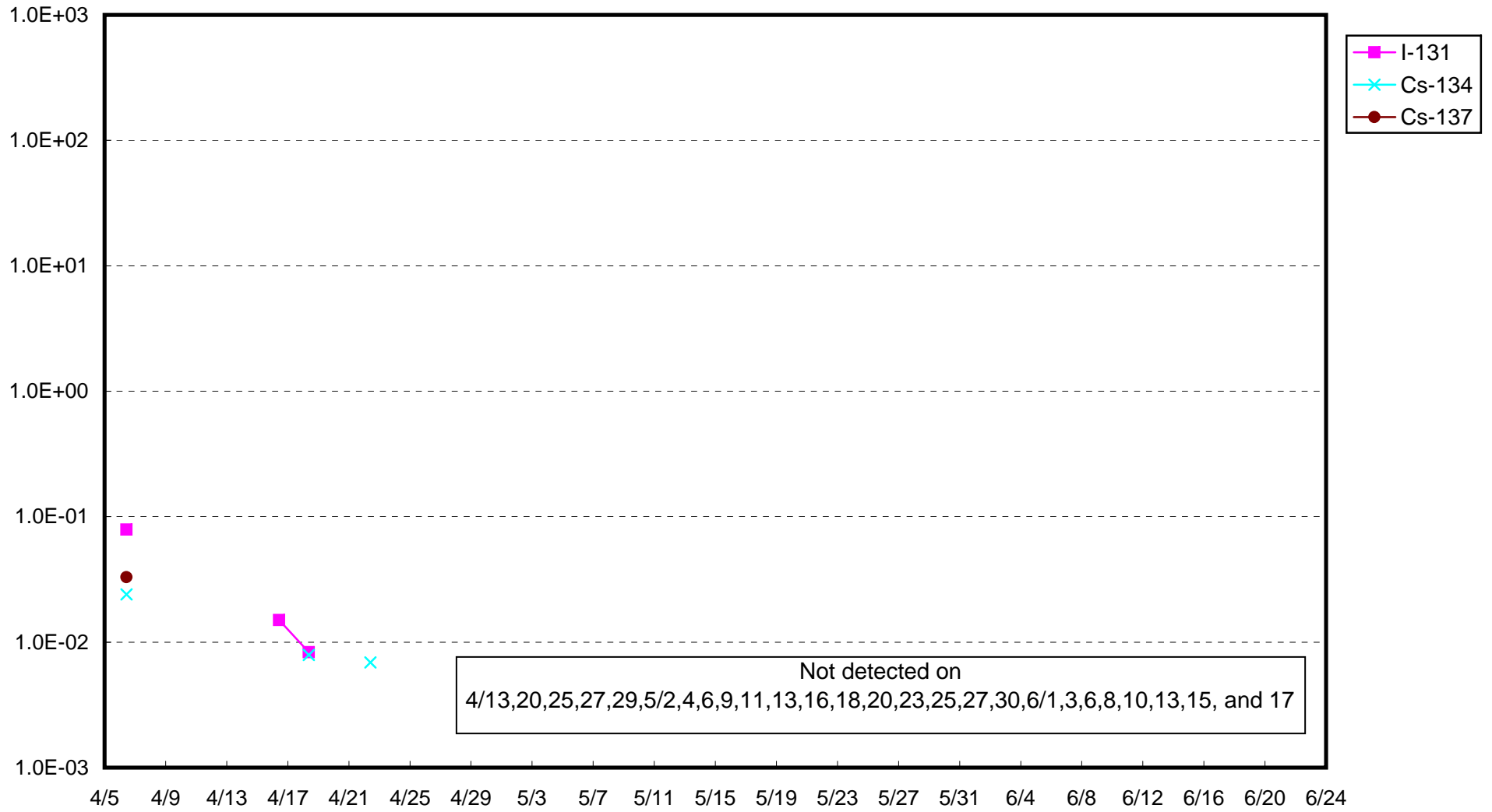
Fukushima Daiich Nuclear Power Station : Radioactivity Density at the Deep Well at the Site (Bq/cm 3 )
