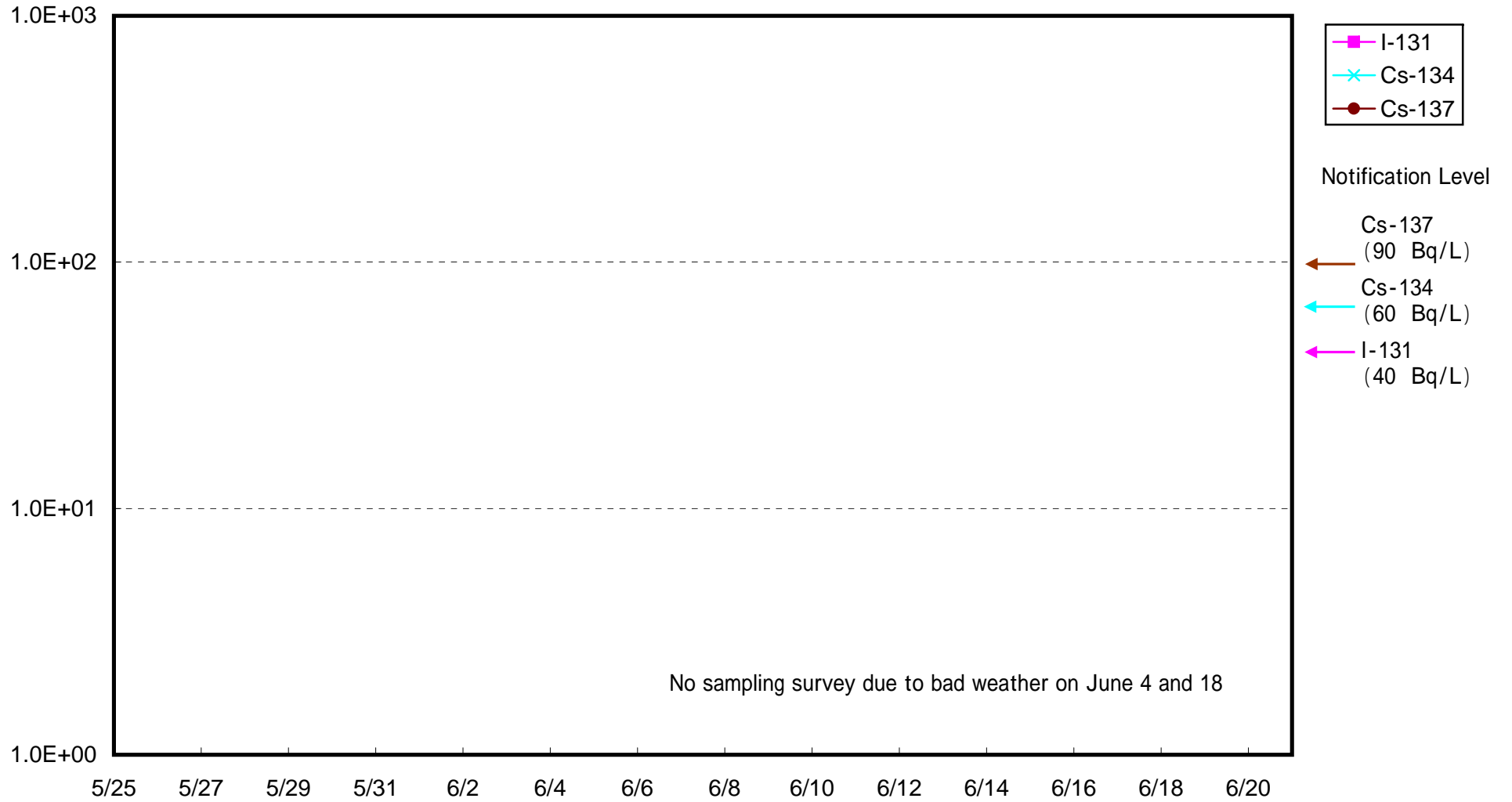
Radioactivity Density of Seawater around approx. 15 km offshore of Fukushima Daini upper layer (Bq/L)
