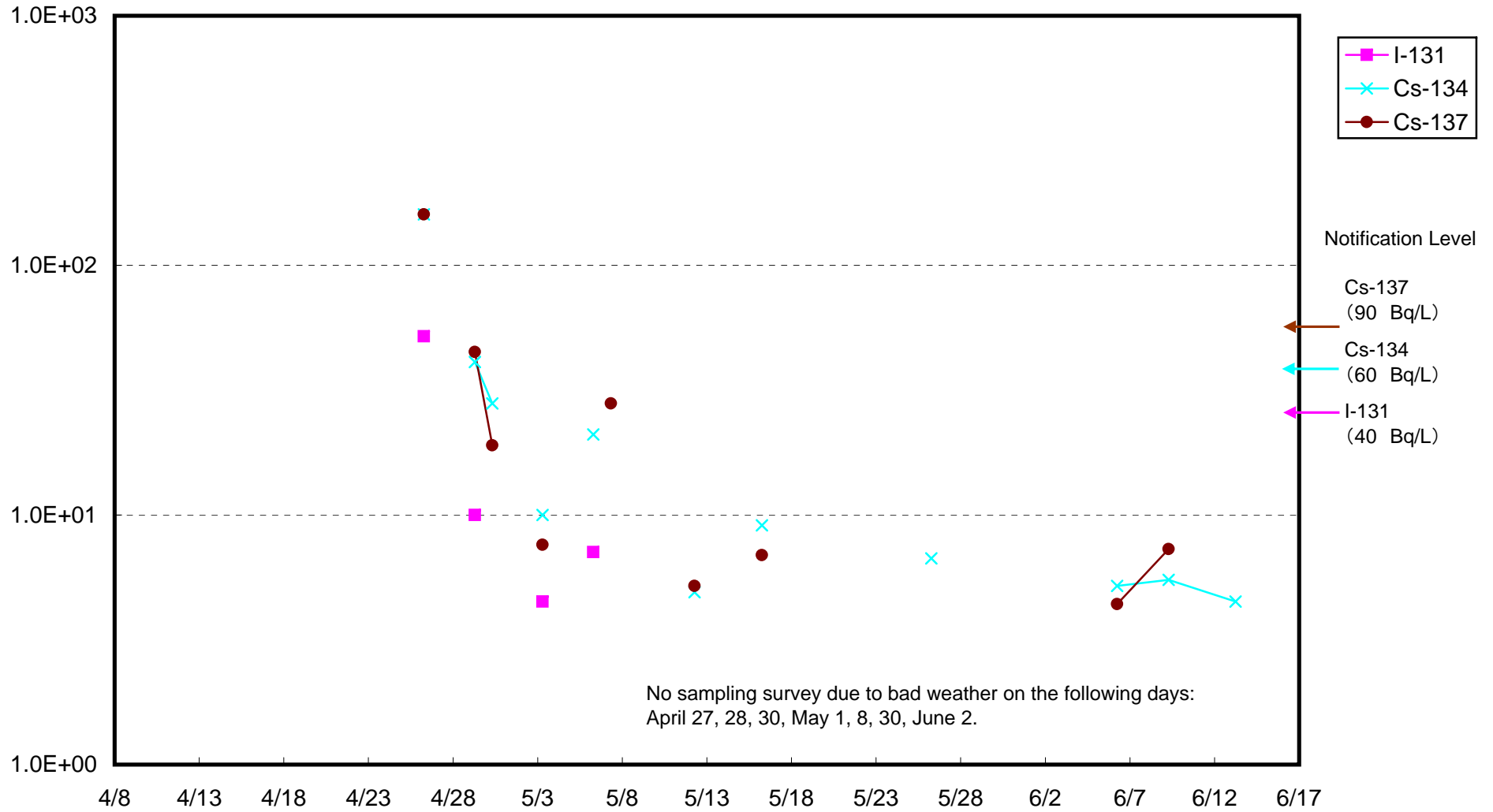
Radioactivity Density of Seawater around 3 km offshore of Natsuigawa, Upper layer (Bq/ L)
