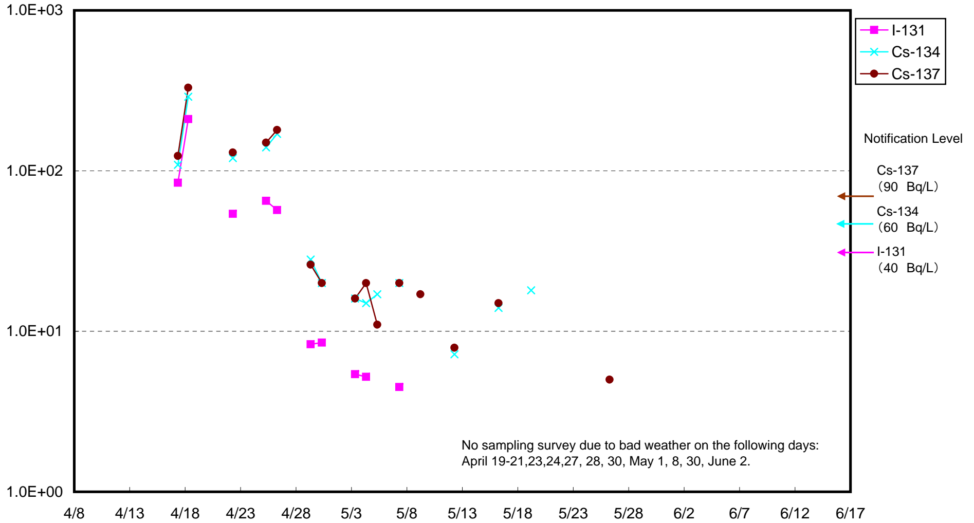
Radioactivity Density of Seawater around 3 km offshore of Northern part of Iwaki City, Upper layer (Bq/ L)
