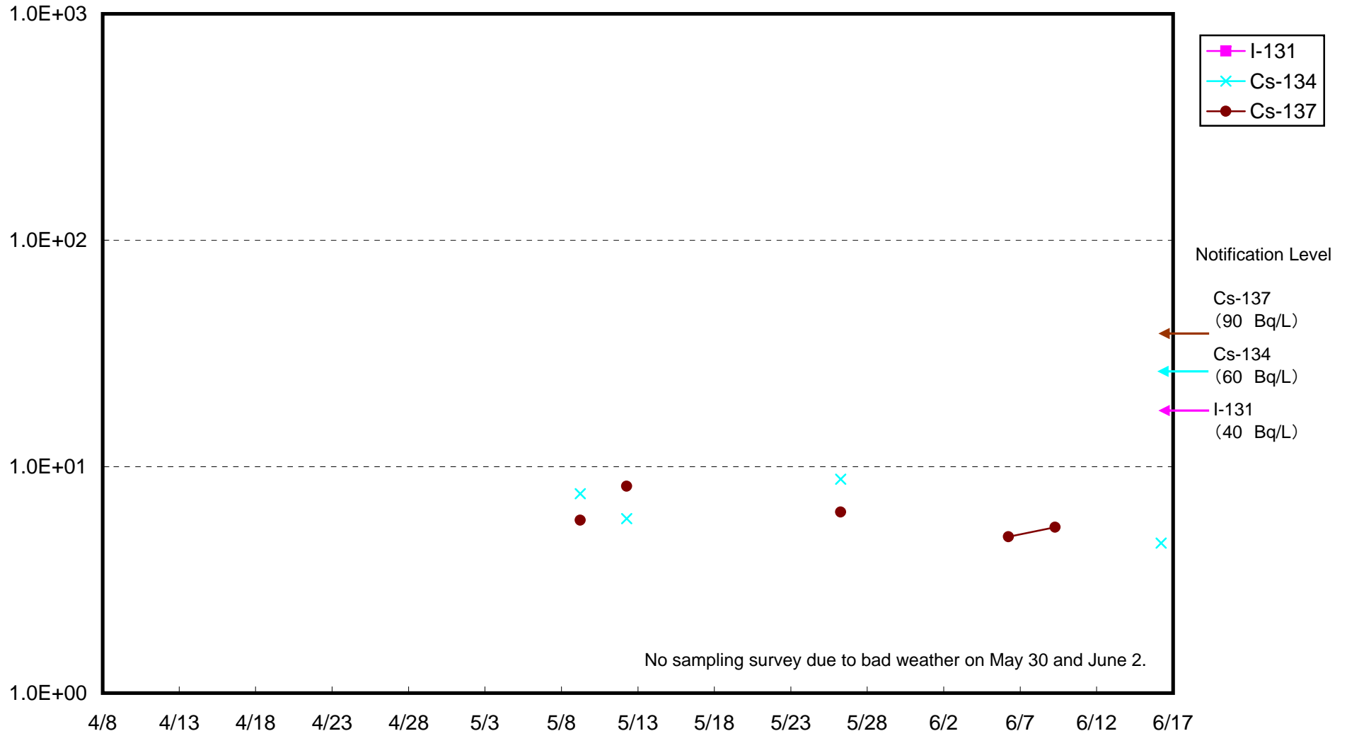
Radioactivity Density of Seawater around 3 km offshore of Natsuigawa, Lower layer (Bq/ L)
