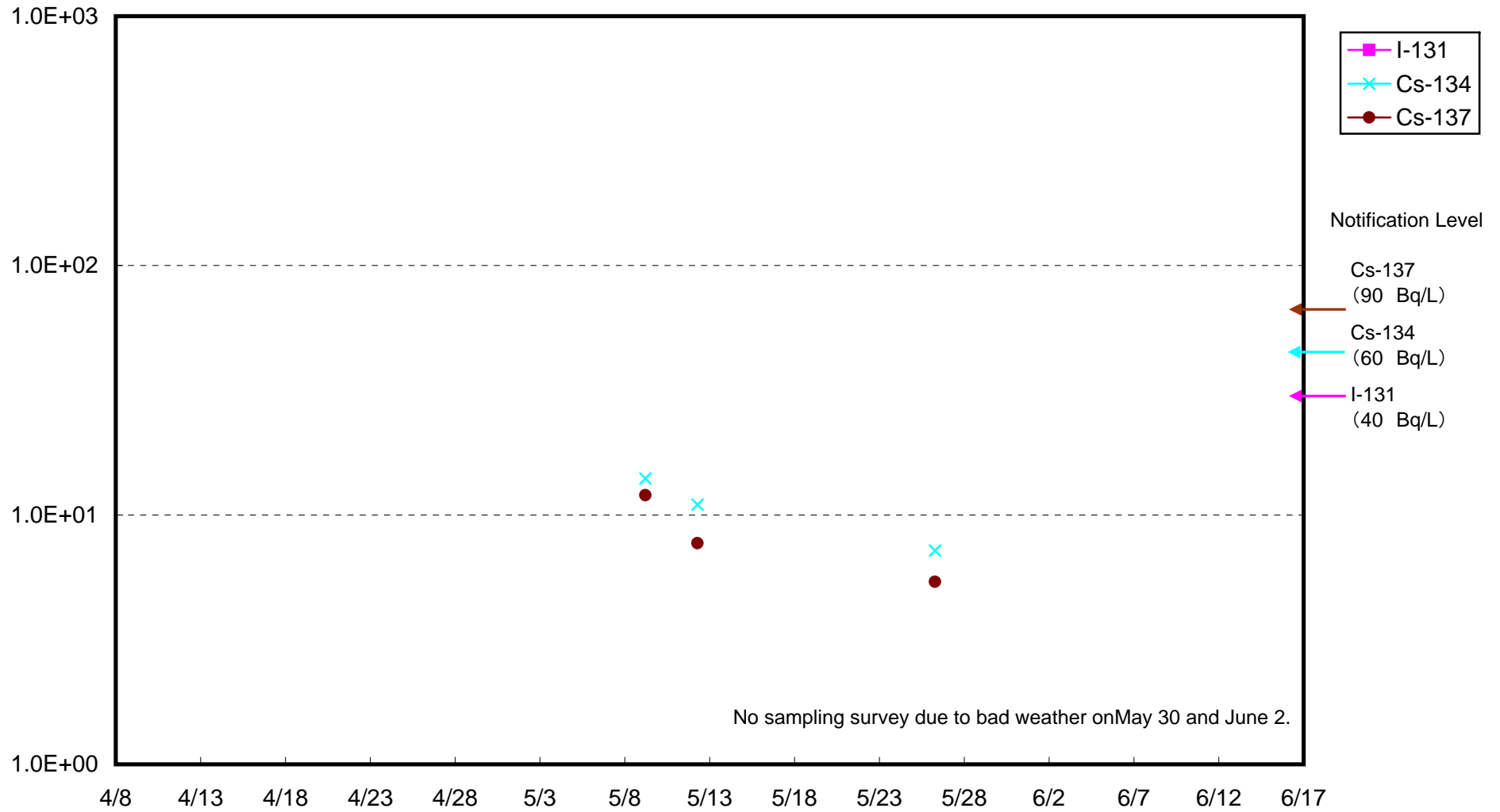
Radioactivity Density of Seawater around 3 km offshore of Northern part of Iwaki City, Lower layer (Bq/ L)
