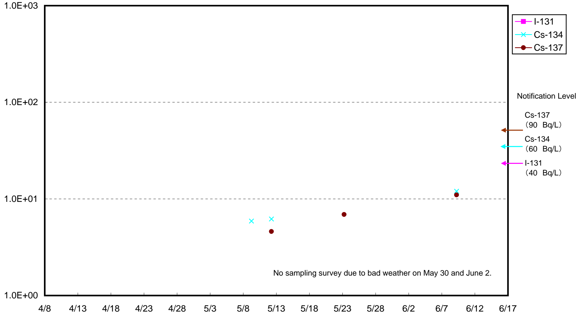
Radioactivity Density of Seawater around 3 km offshore of Numanouchi, Lower layer (Bq/ L)
