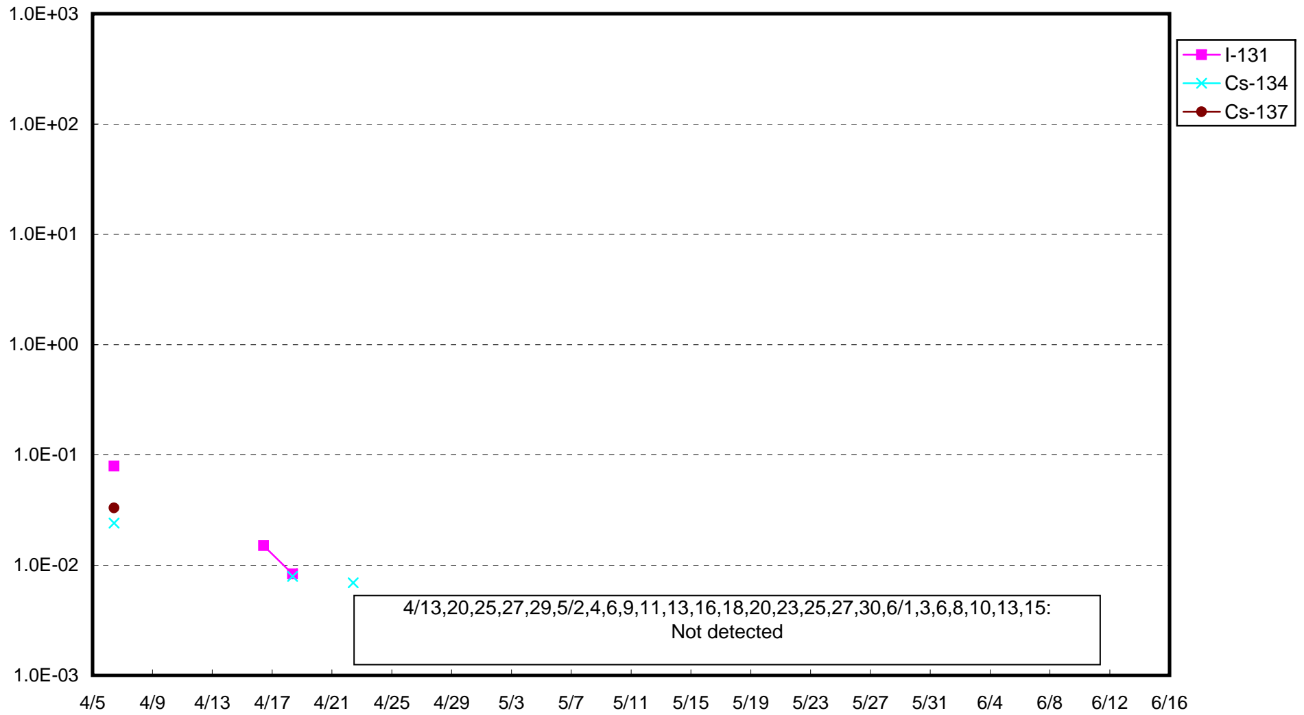
Fukushima Daiichi Nuclear Power Station : Radioactivity Density of Deep Wells at the Site (Bq/cm 3 )
