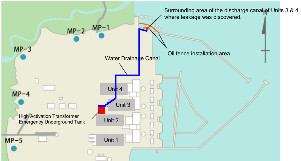
Figure depicting status of oil leakage in the surroundings of the discharge channels of Units 3 and 4
