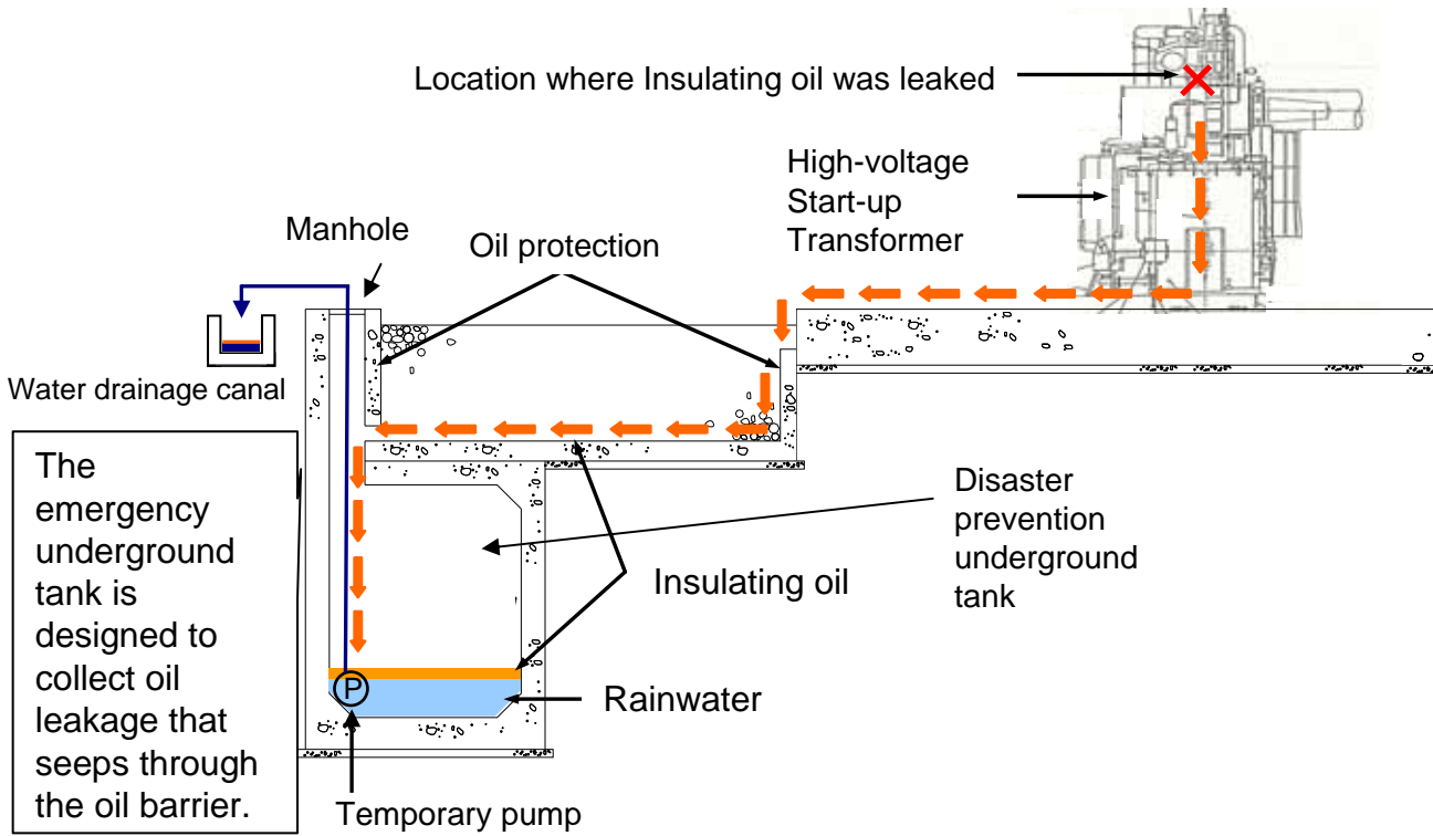
Oil leakage conditions of High-voltage Start-up Transformer
