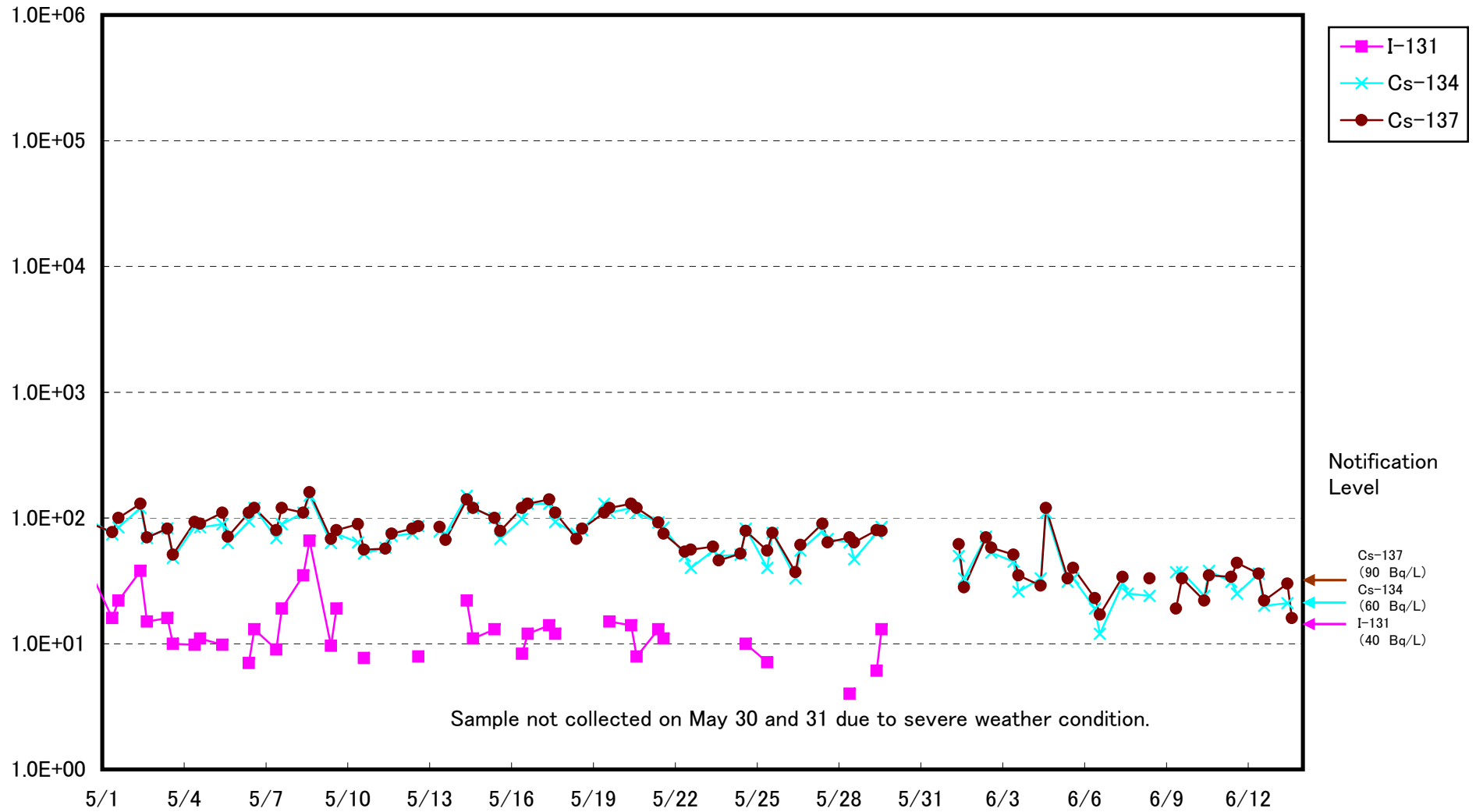
Radioactivity Density of Seawater at North of 1F5-6 Discharge Channel (approx.30m north of 5-6 discharge channel)
