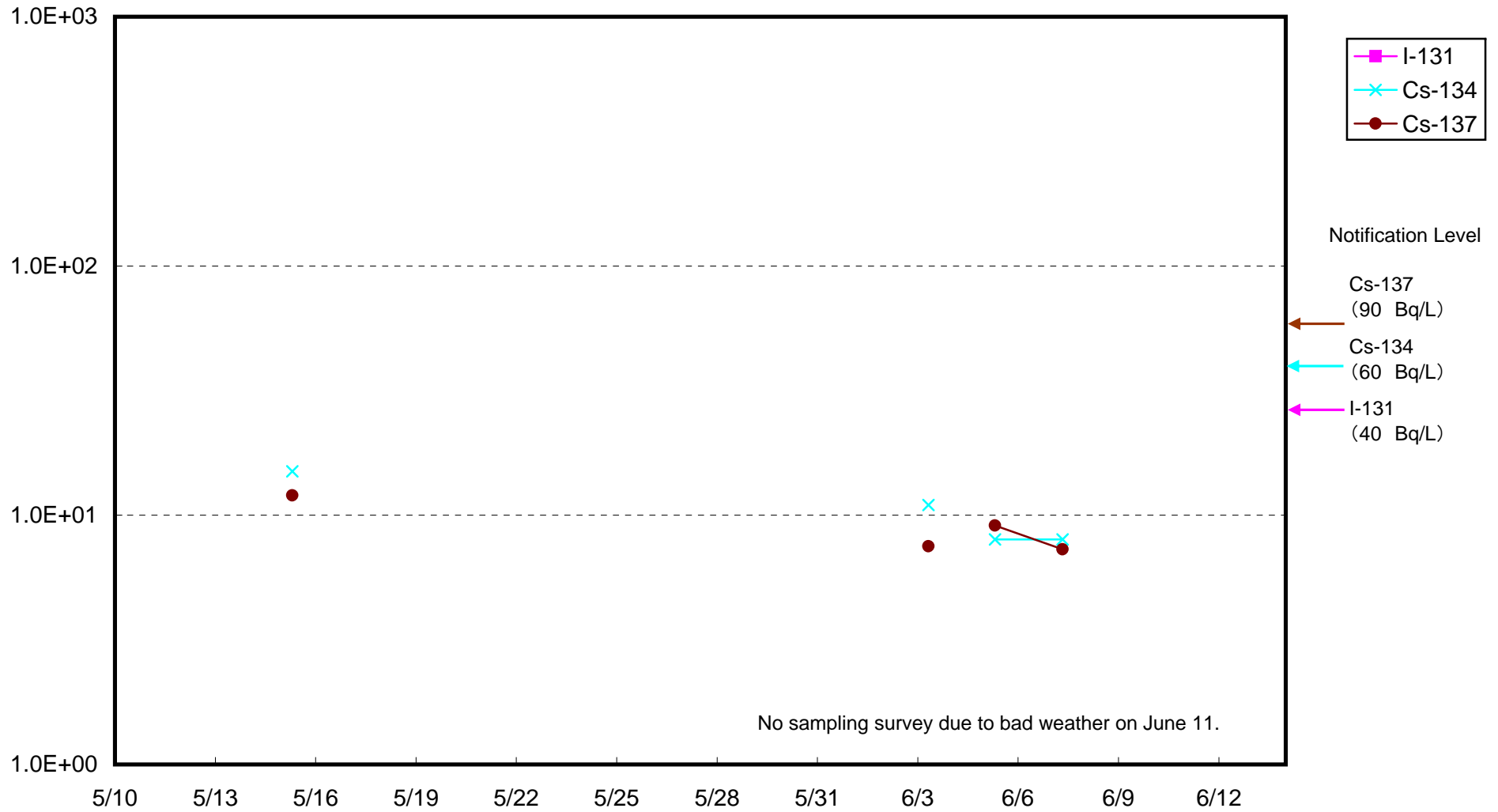
Radioactivity Density of Seawater around 3 km offshore of Iwasawa Shore Lower layer (Bq/ L)
