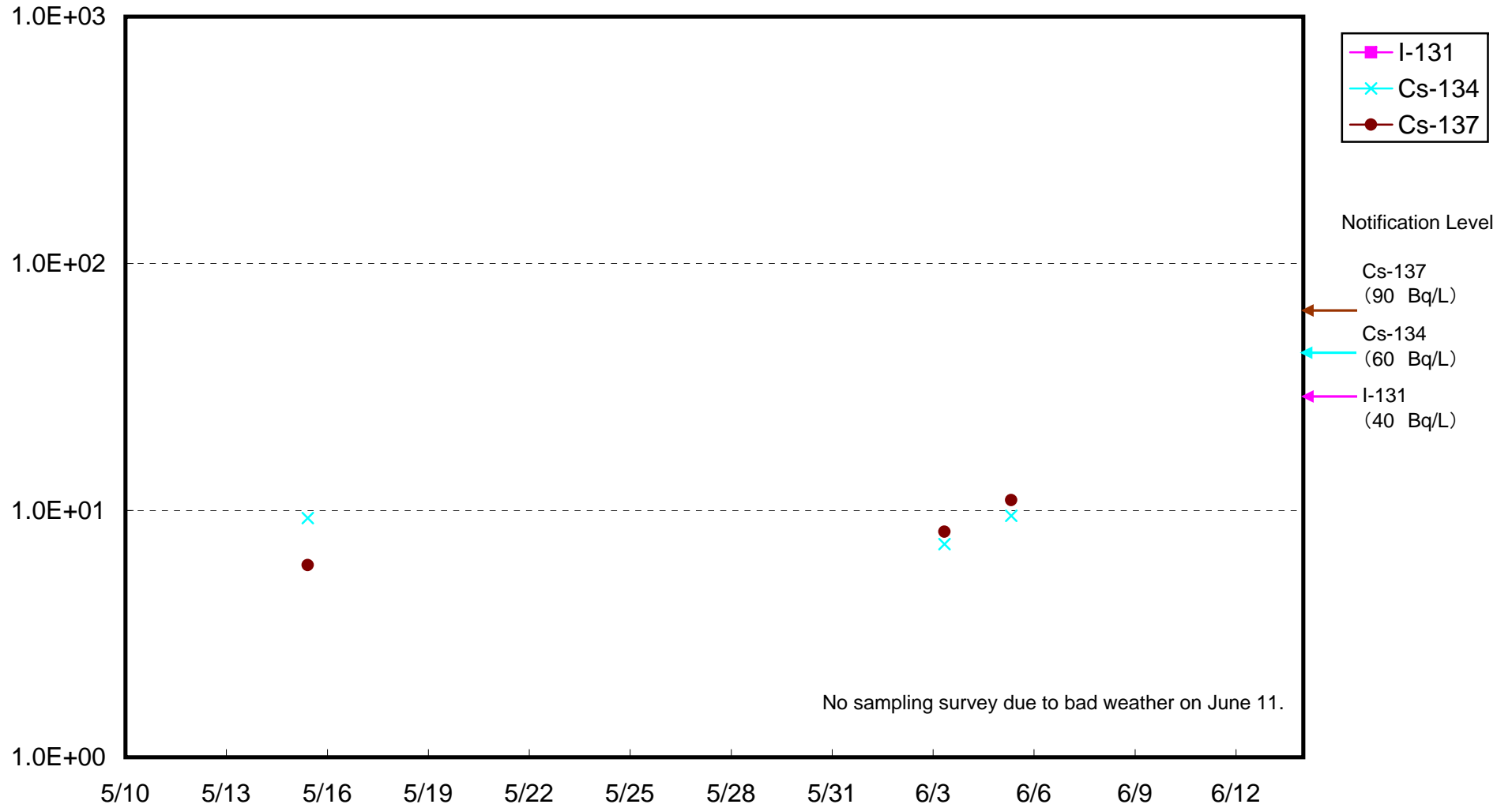
Radioactivity Density of Seawater around 8 km offshore of Iwasawa Shore Lower layer (Bq/ L)
