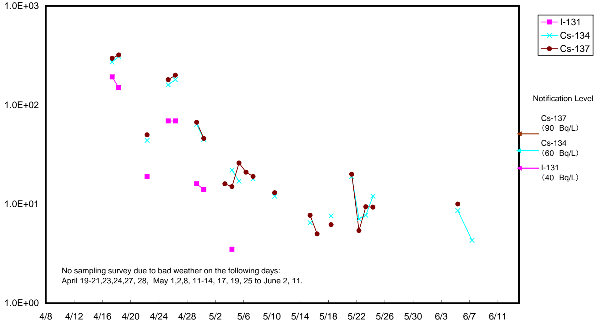
Radioactivity Density of Seawater around 8 km offshore of Iwasawa Shore Upper layer (Bq/ L)
