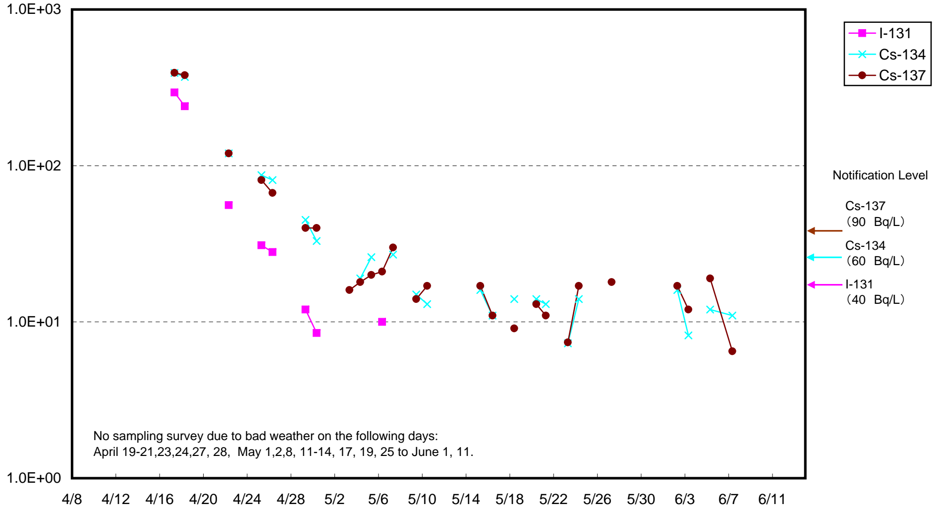
Radioactivity Density of Seawater around 3 km offshore of Iwasawa Shore Upper layer (Bq/ L)
