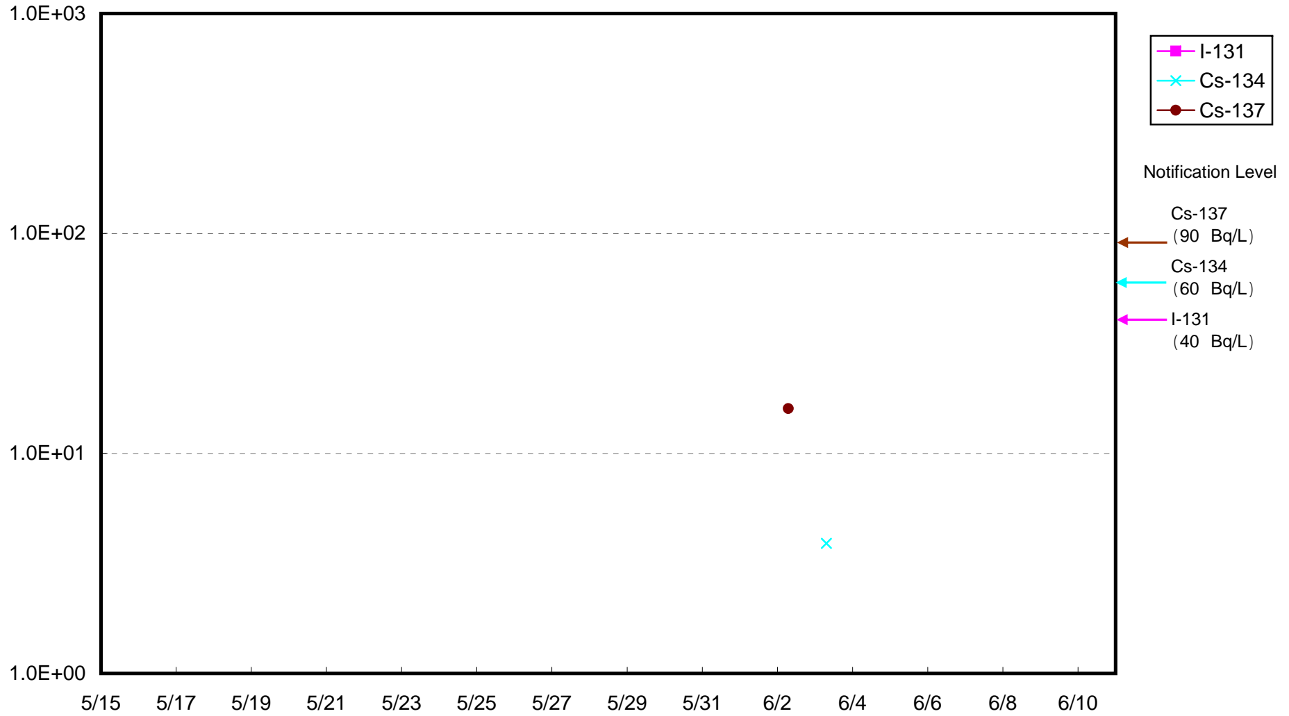
沼Radioactivity Density of Seawater around approx. 5km offshore of Numanouchi Lower layer (Bq/L)
