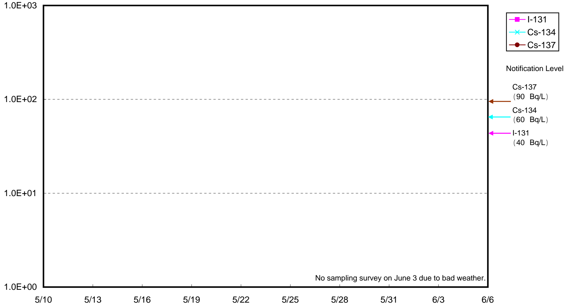
Radioactivity Density of Seawater around 8 km offshore of Odaka-ku Lower layer (Bq/L)
