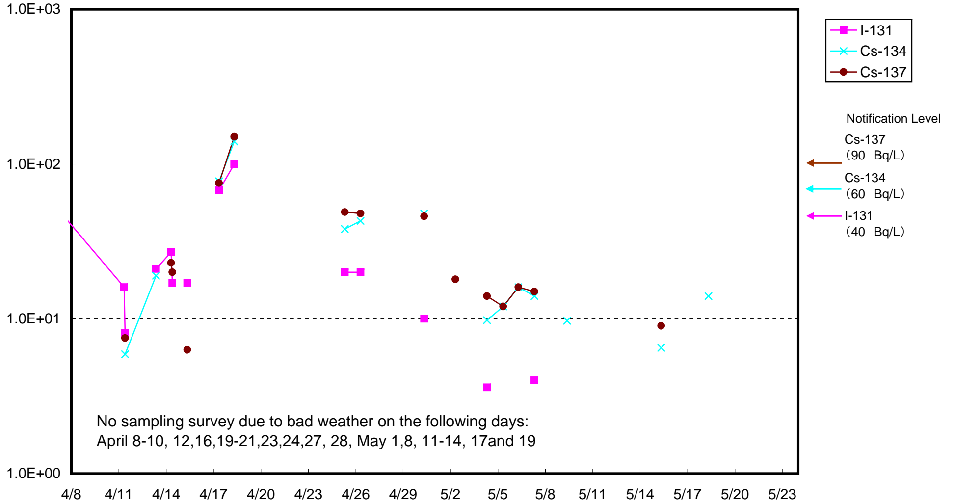
Radioactivity Density of Seawater around approx. 15 km offshore of Hirono town (Bq/L)
