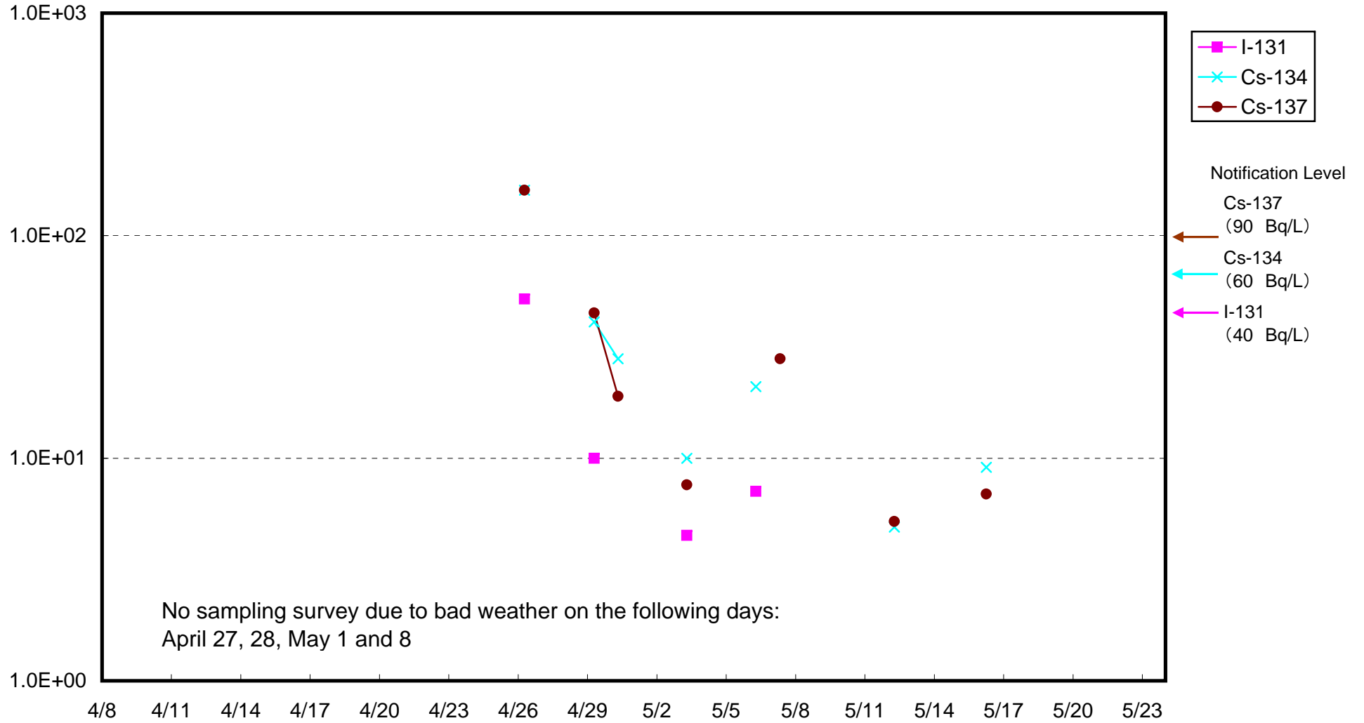
Radioactivity Density of Seawater around 3 km offshore of Natsui River (Bq/L) (upper layer)
