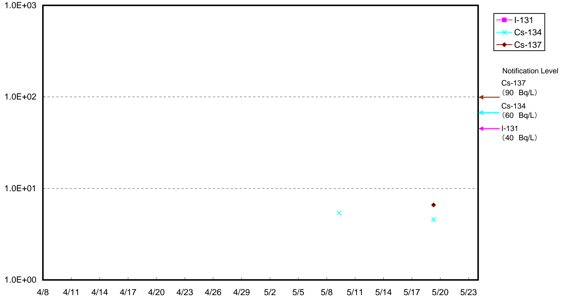
Radioactivity Density of Seawater around 3 km offshore of Ena (Bq/L) (lower layer)
