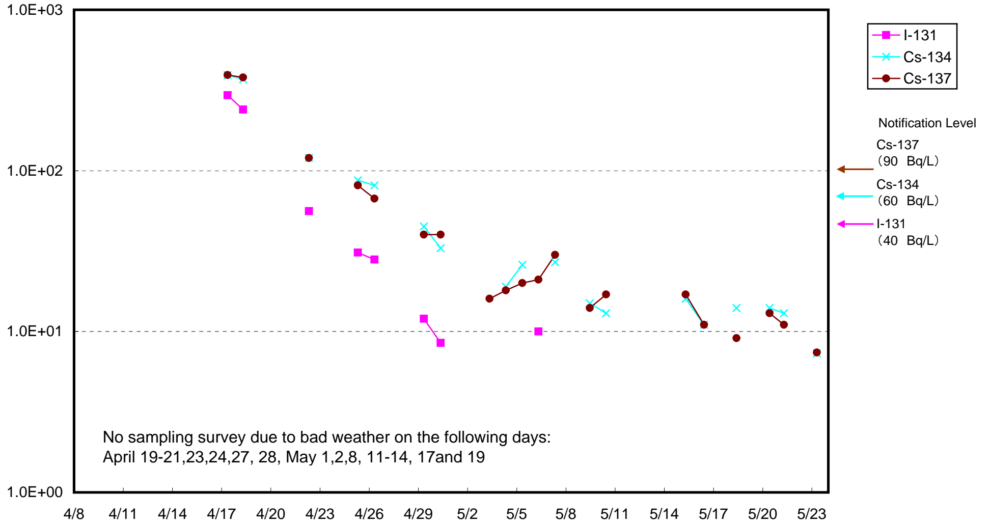
Radioactivity Density of Seawater around approx. 3km offshore of Iwasawa Shore (Bq/L) (upper layer)
