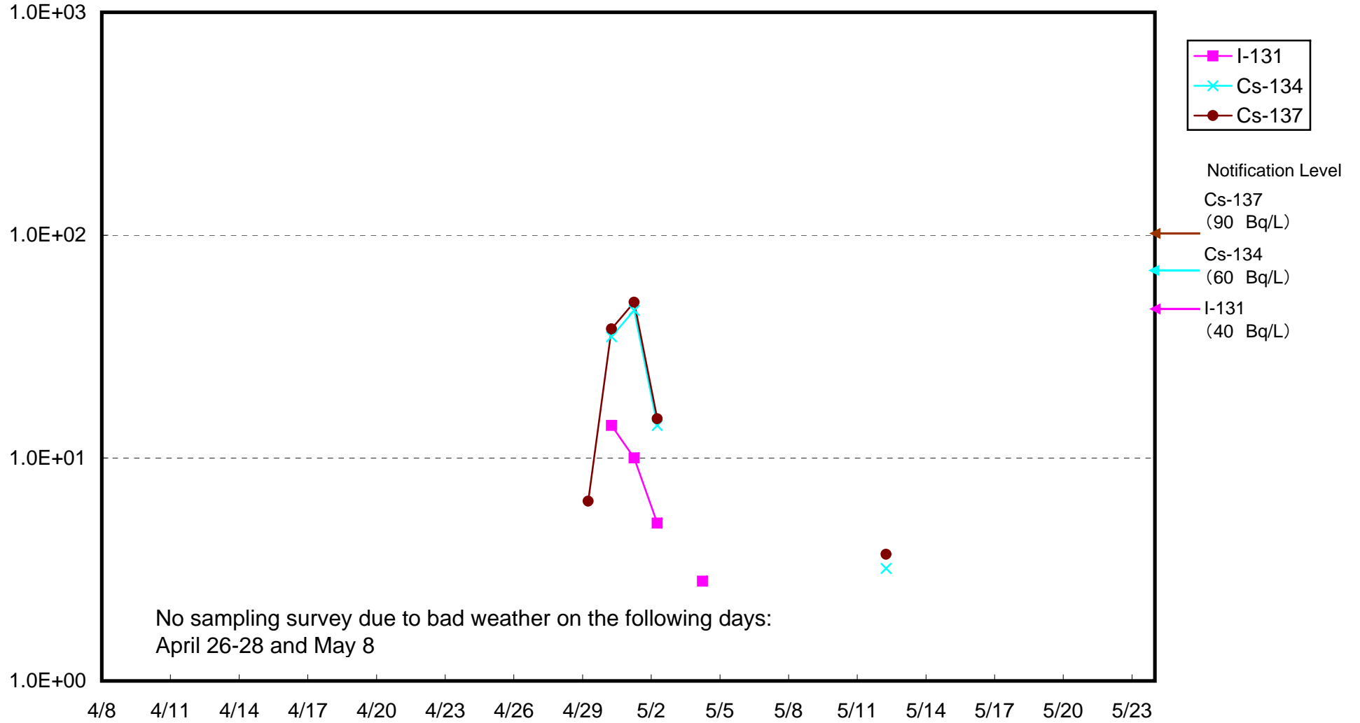
Radioactivity Density of Seawater around 3 km offshore of Onahama Port (Bq/L) (upper layer)
