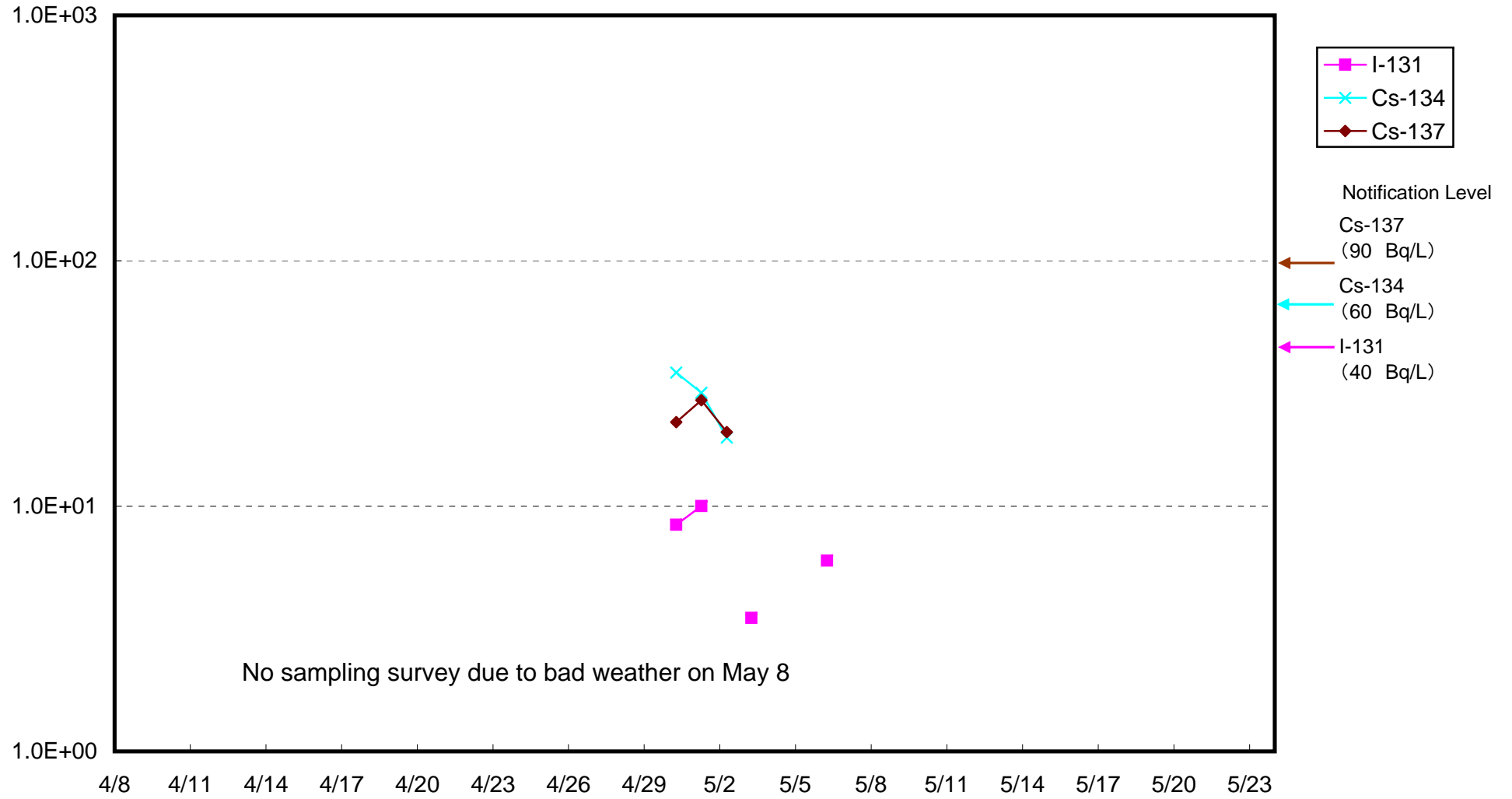
Radioactivity Density of Seawater around 3 km offshore of Ena (Bq/L) (upper layer)
