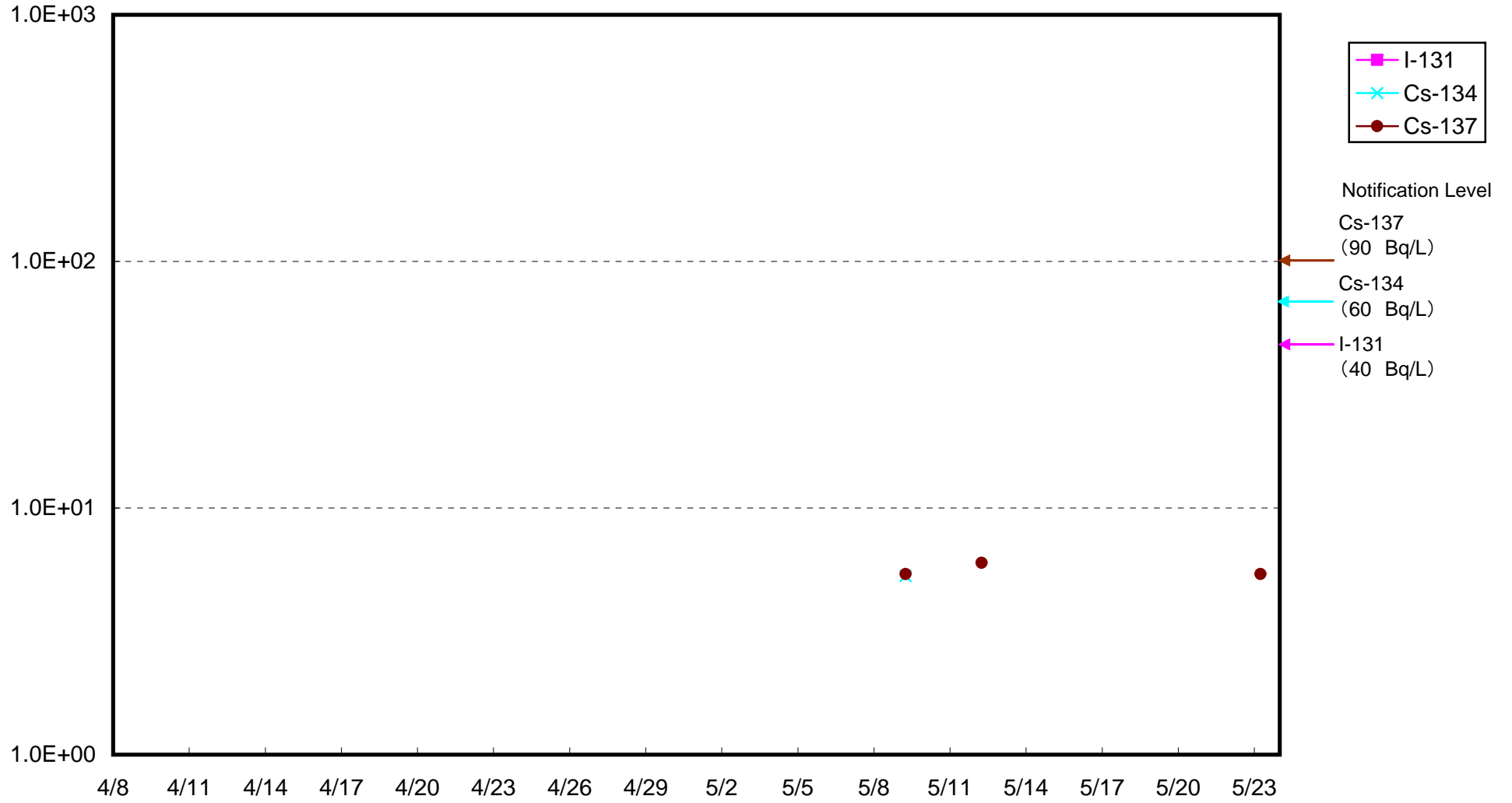
Radioactivity Density of Seawater around 3 km offshore of Toyoma (Bq/L) (Lower layer)
