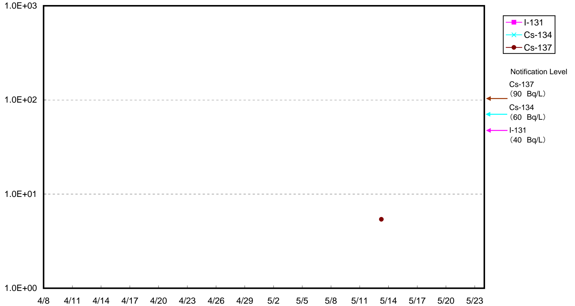
Radioactivity Density of Seawater around 3 km offshore of Onahama Port (Bq/L) (Lower layer)
