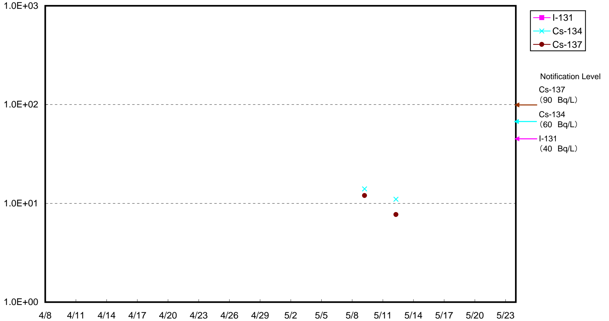
Radioactivity Density of Seawater around 3 km offshore of Northern Part of Iwaki City (Bq/L) (lower layer)
