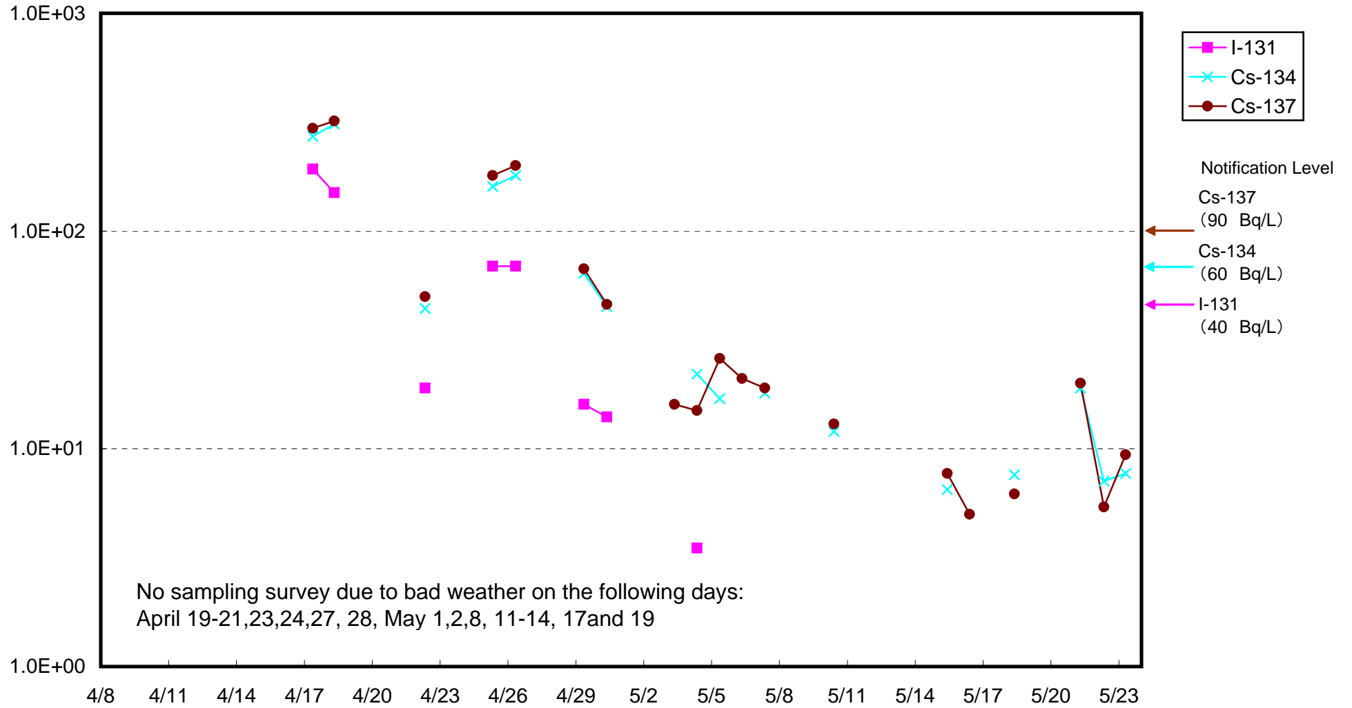
Radioactivity Density of Seawater around approx. 8km offshore of Iwasawa Shore (Bq/L) (upper layer)
