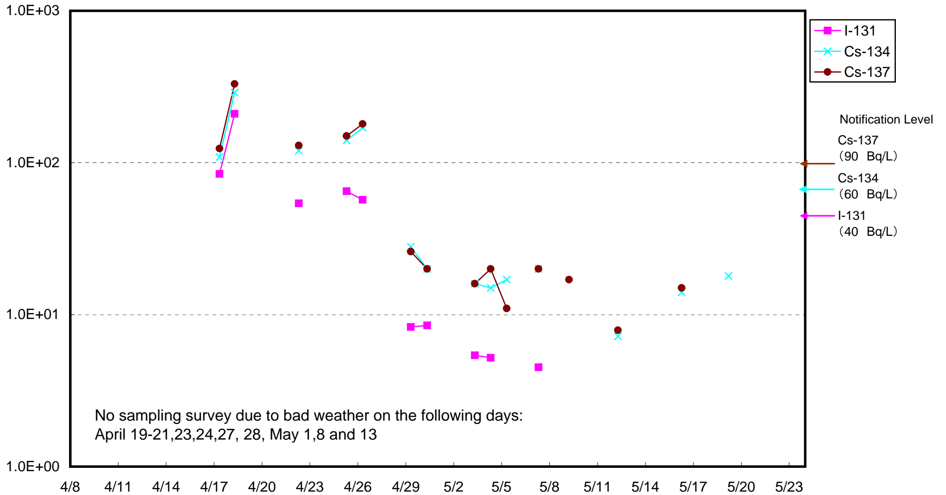
Radioactivity Density of Seawater around 3 km offshore of Northern Part of Iwaki City (Bq/L) (Upper layer)
