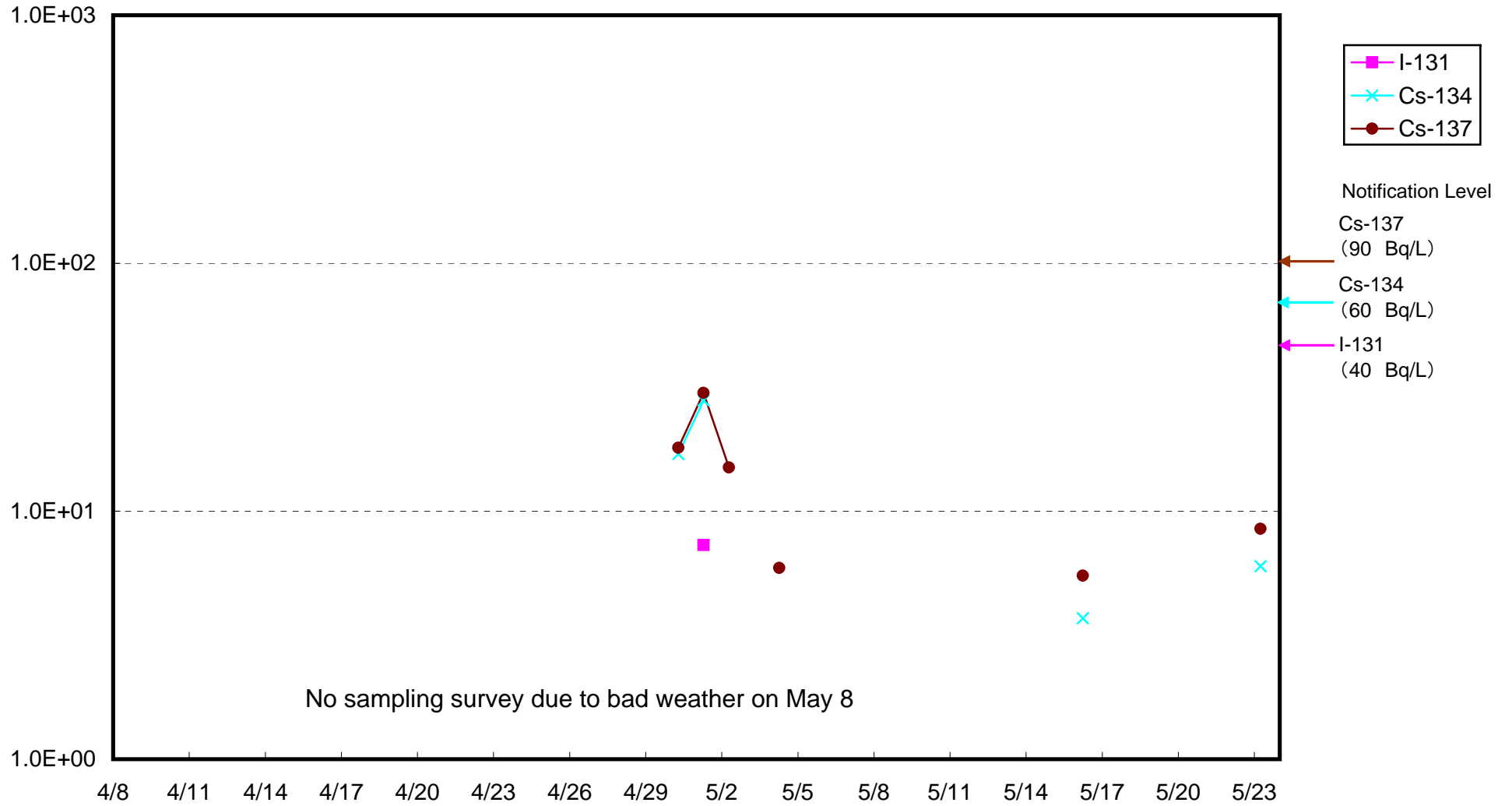
Radioactivity Density of Seawater around 3 km offshore of Toyoma (Bq/L) (upper layer)
